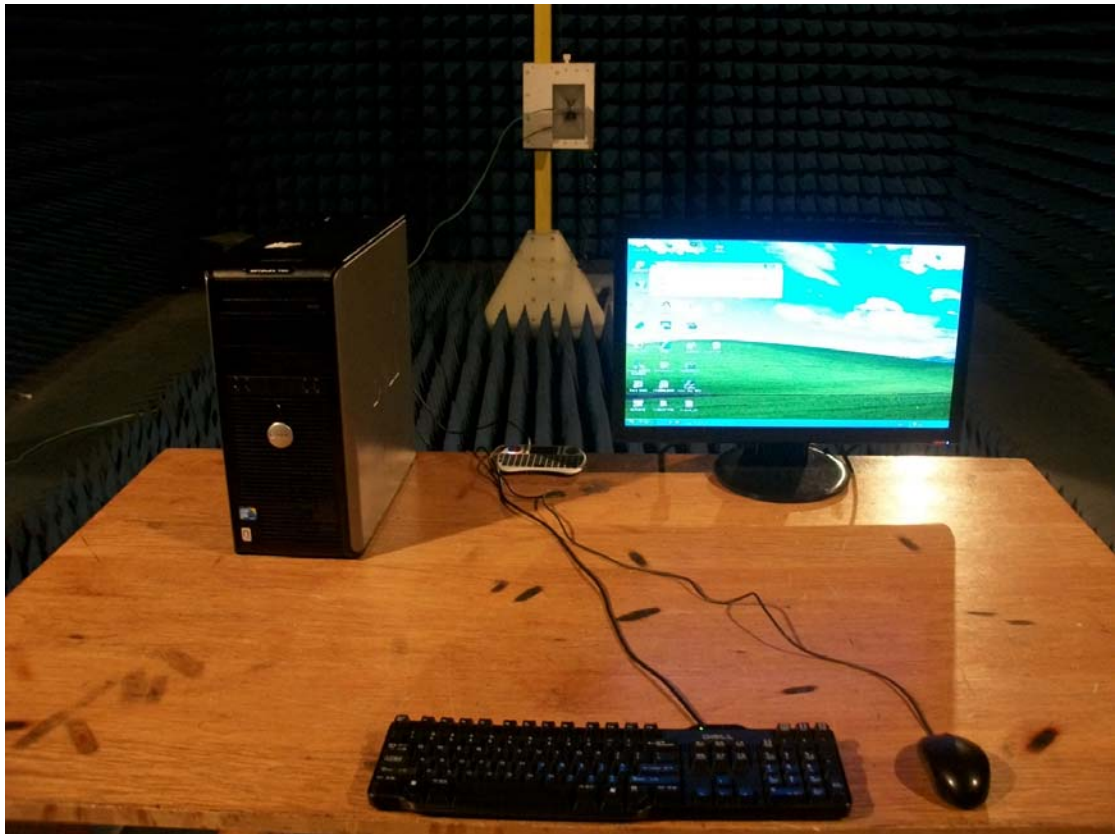
Test photo of radiated emission( f > 1\text{GHz} )
