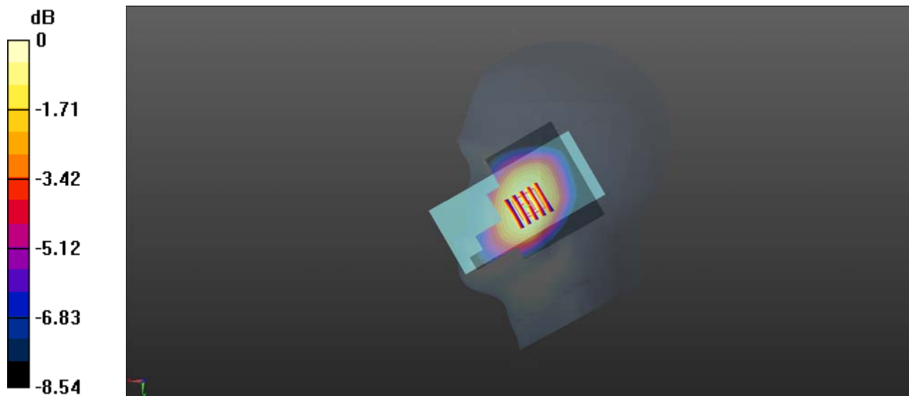
0 dB = 0.305 W/kg
