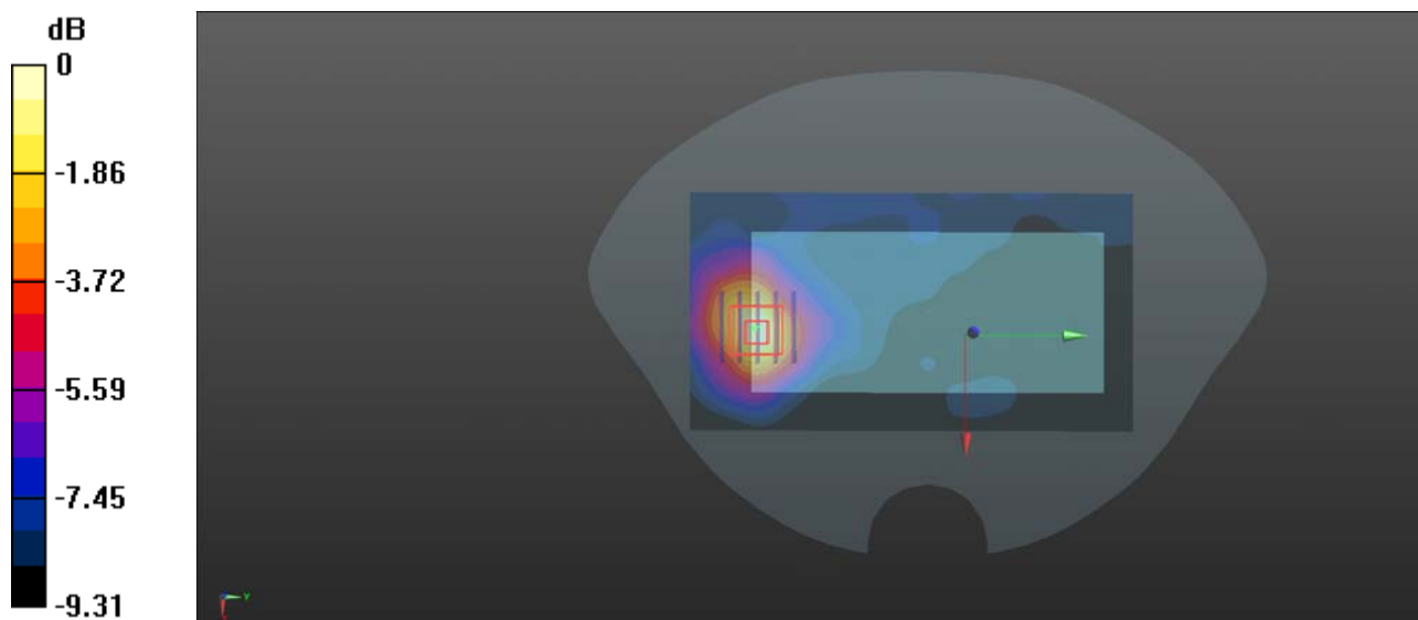
0 dB = 0.364 W/kg
