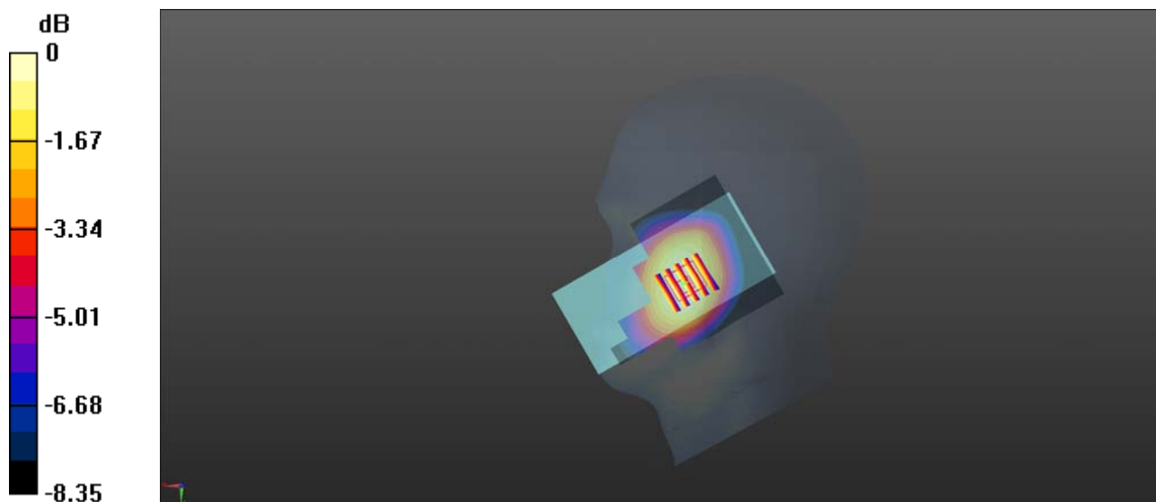
0 dB = 0.163 W/kg
