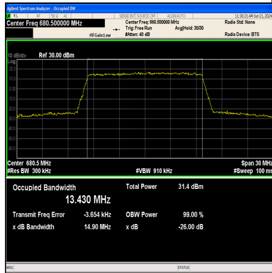
Band71-15MHz-64QAM-133297-75RB#0-PASS
