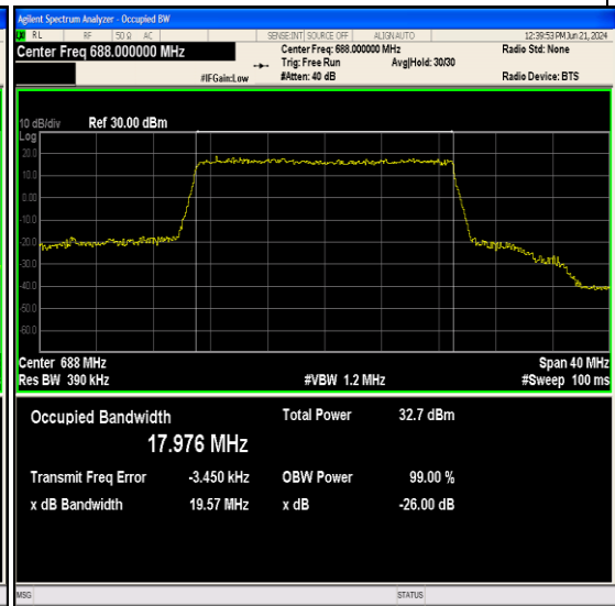
Band71-20MHz-16QAM-133372-100RB#0-PASS
