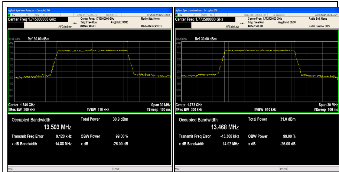
Band66-15MHz-64QAM-132322-75RB#0-PASS
