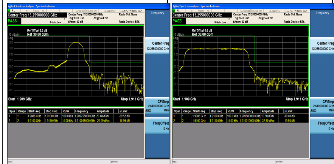
Band2_1.4MHz_16QAM_19193_1RB#5
