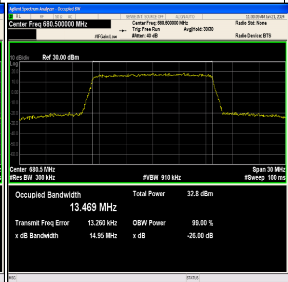
Band71-15MHz-16QAM-133297-75RB#0-PASS
