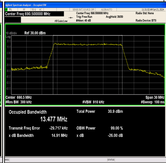
Band71-15MHz-64QAM-133397-75RB#0-PASS
