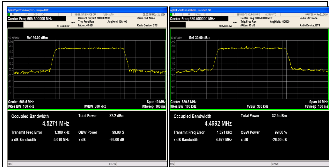
Band71-5MHz-16QAM-133147-25RB#0-PASS
