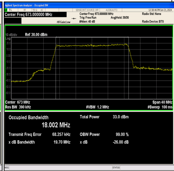
Band71-20MHz-16QAM-133222-100RB#0-PASS
