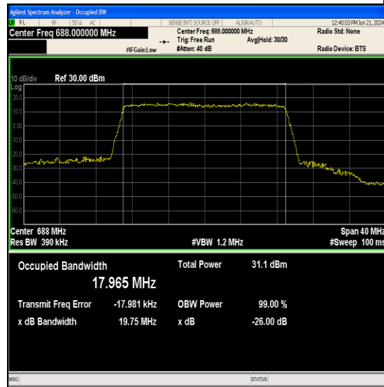
Band71-20MHz-64QAM-133372-100RB#0-PASS
