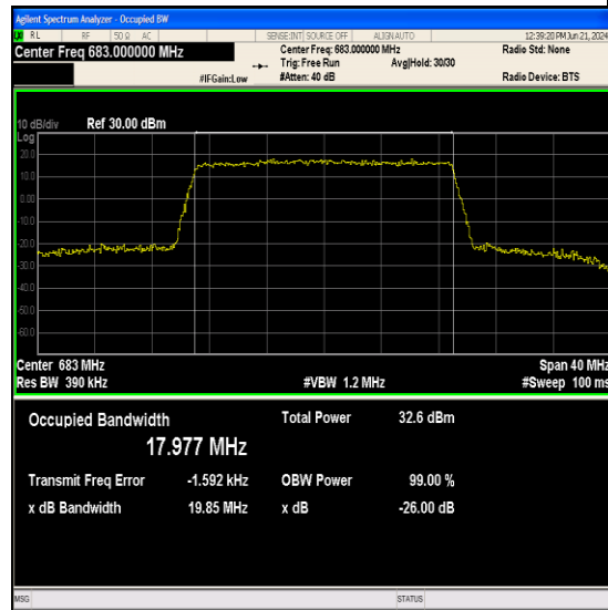
Band71-20MHz-16QAM-133322-100RB#0-PASS
