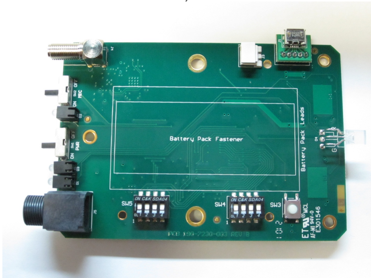
Battery Side
