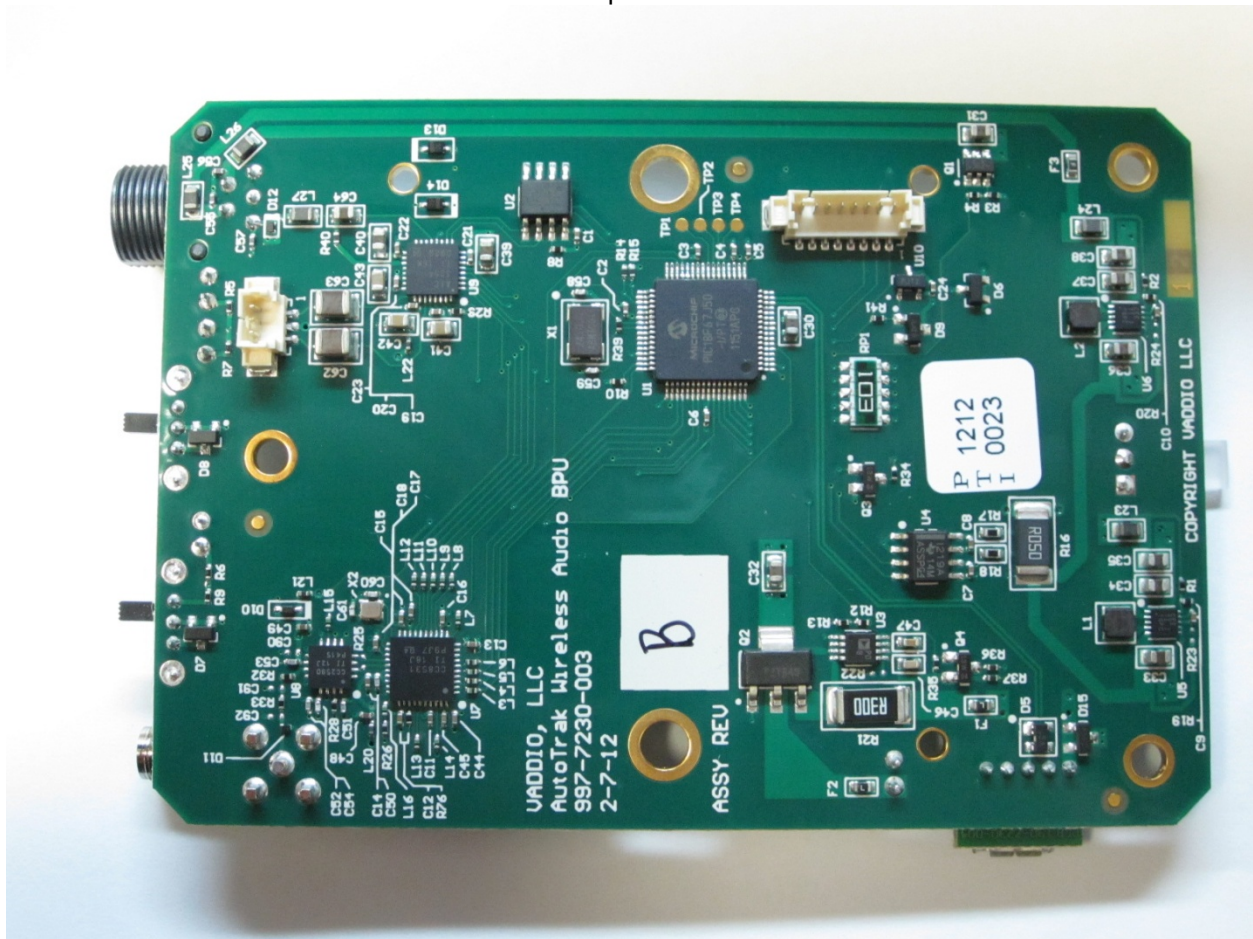
Chip Side
