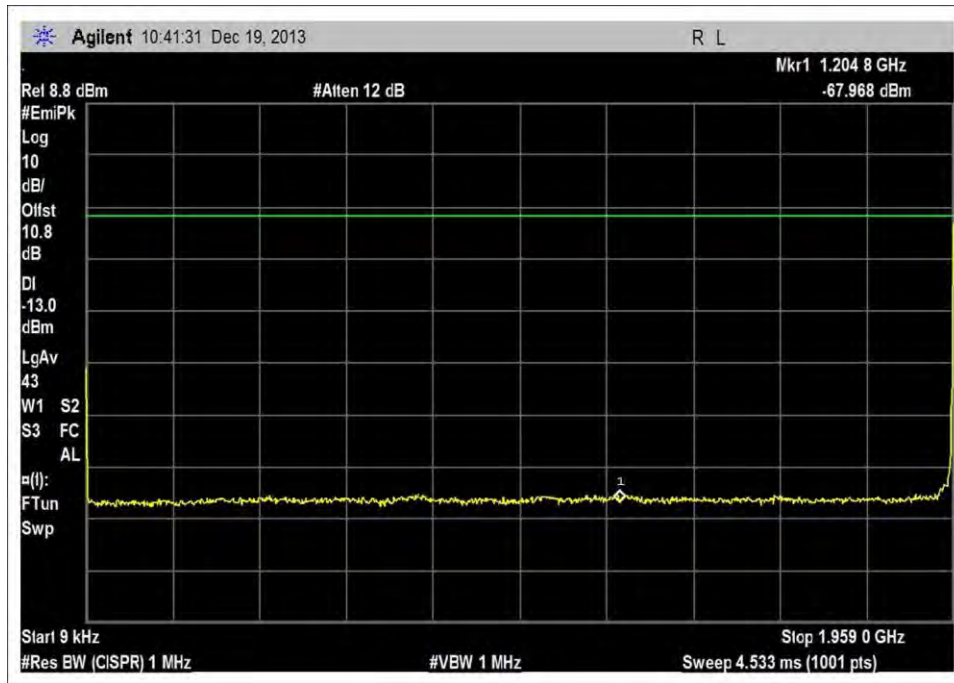
DL_1930-1995MHz_M_4.1AWGN_1
