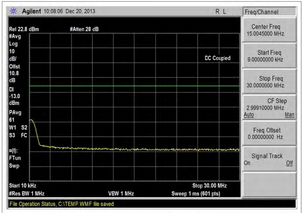
UL_1850-1915MHz_M_5WCDMATM1_1
