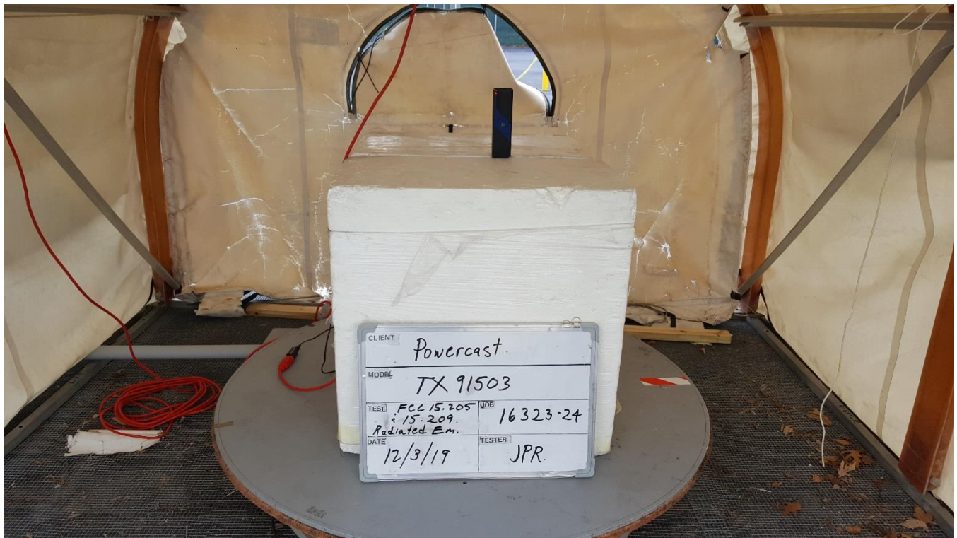
Photograph 1: Radiated Emissions Test Configuration – Upright
