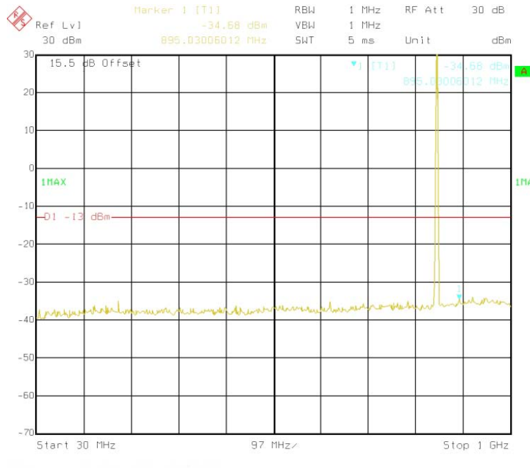
(Plot C1:GSM 850MHz Channel = 251, 30MHz to 1GHz)
