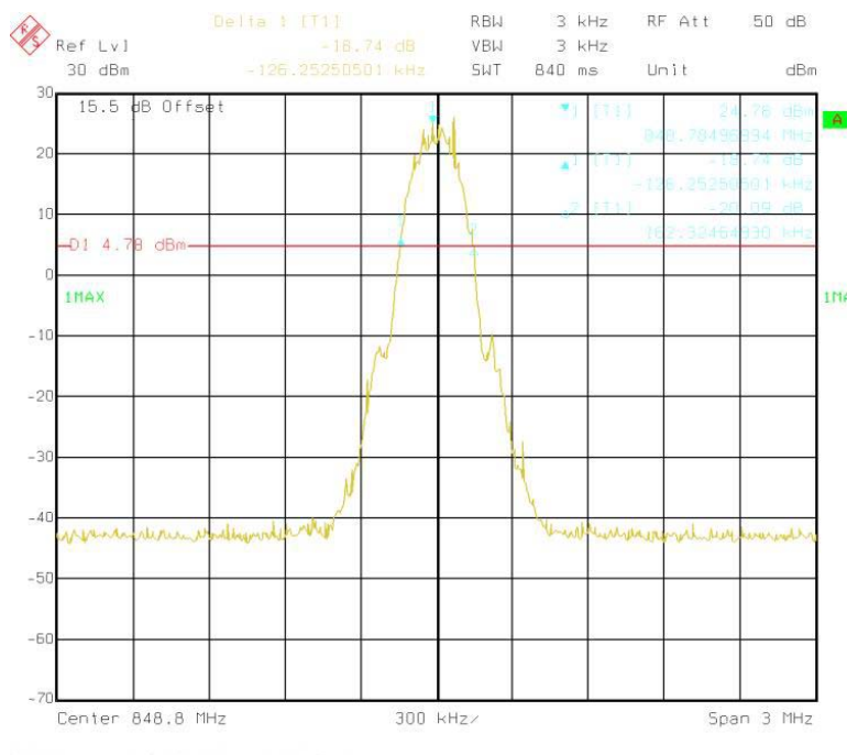
(Plot C1:GSM 850MHz Channel = 251)
