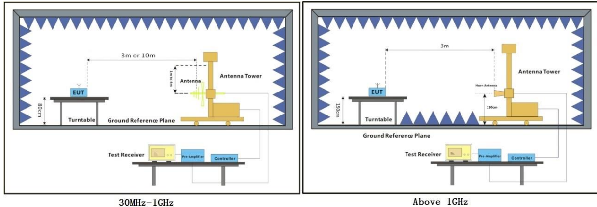
30MHz-1GHz
