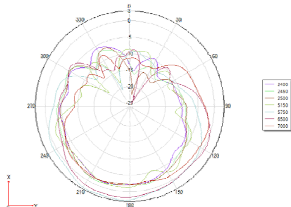
Theta 90°
