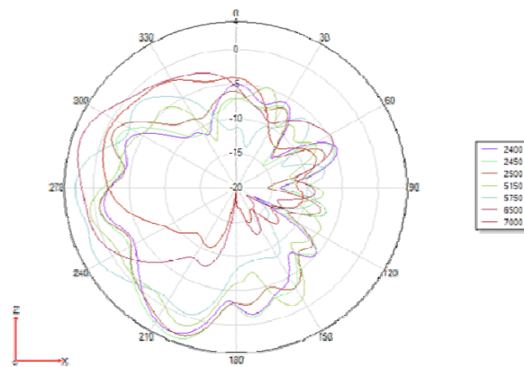
Phi 0°
