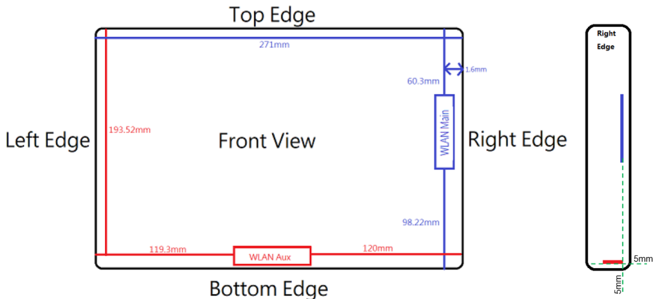
Photograph 17. Antenna position of EUT
