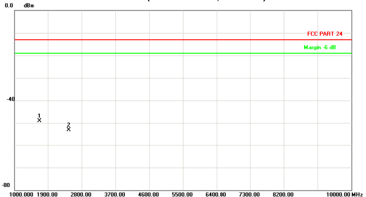
TX CH4233(Above 1000 MHz, Horizontal)
