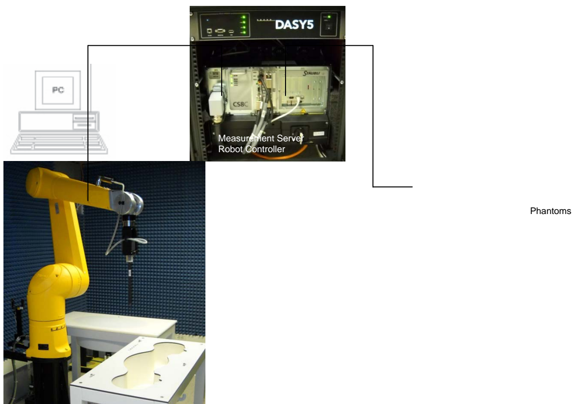
Figure 5: Schematic diagram of the SAR measurement system
