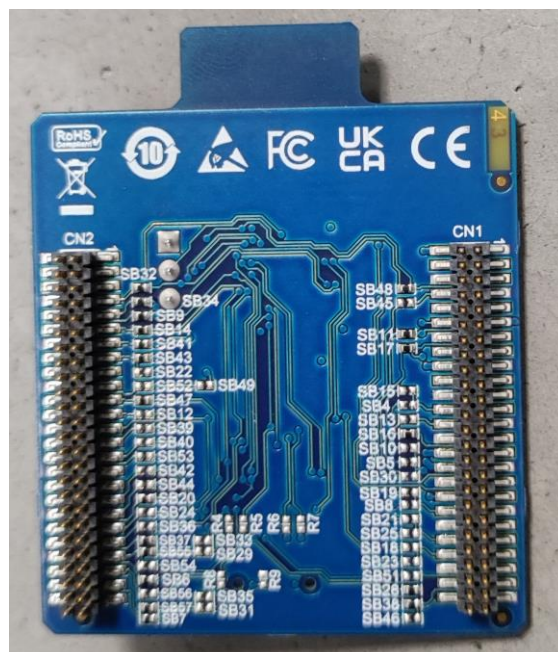
Rear side of MB2032B
