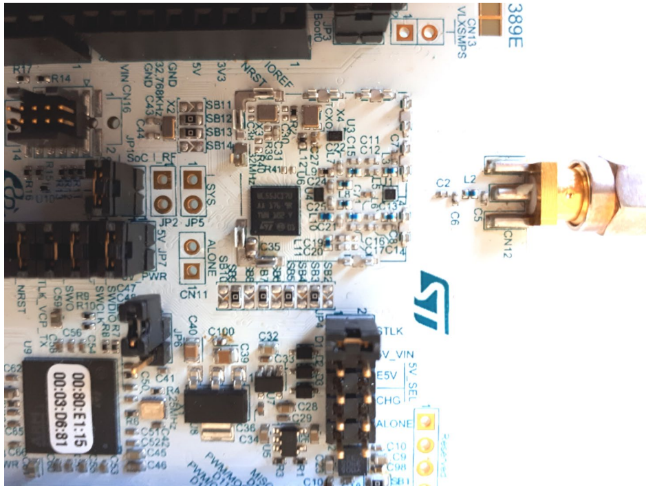
Shield removed
