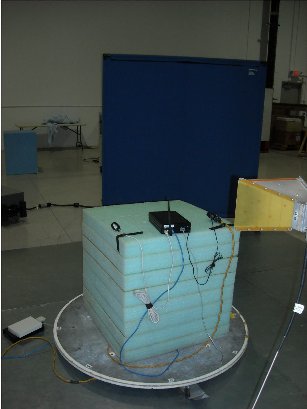
Radiated Measurements Above 1GHz
