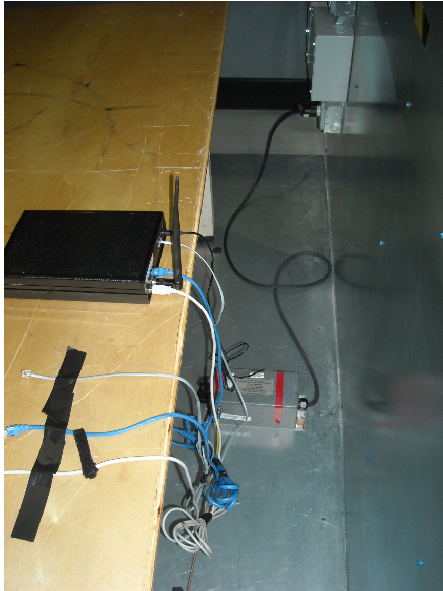
AC mains Line Conducted Measurements - Rear
