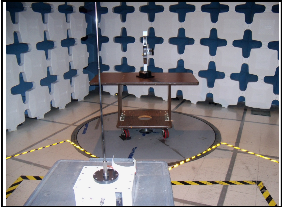
Radiated Emission Setup Photo # 1
