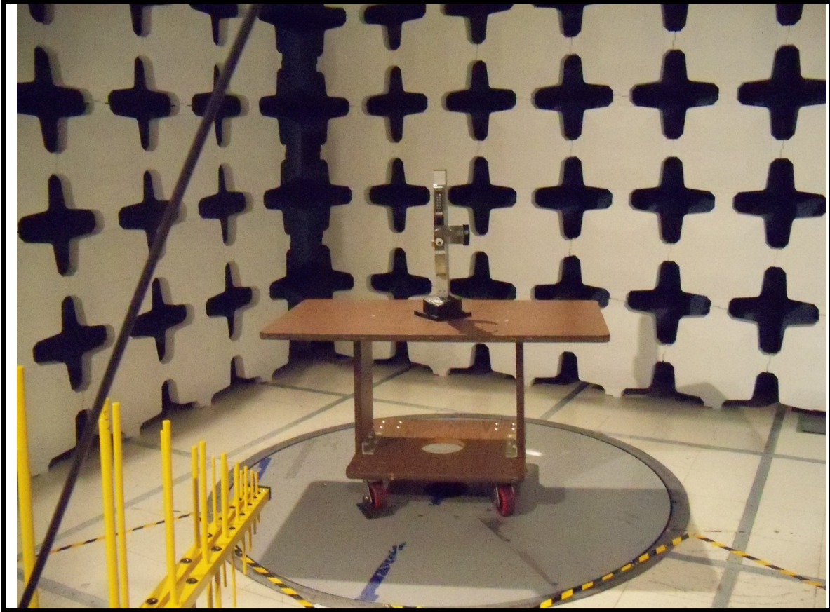
Radiated Emission Setup Photo # 2
