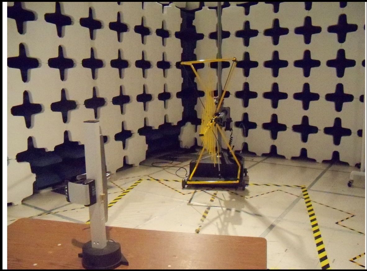
Radiated Emission Setup Photo # 3
