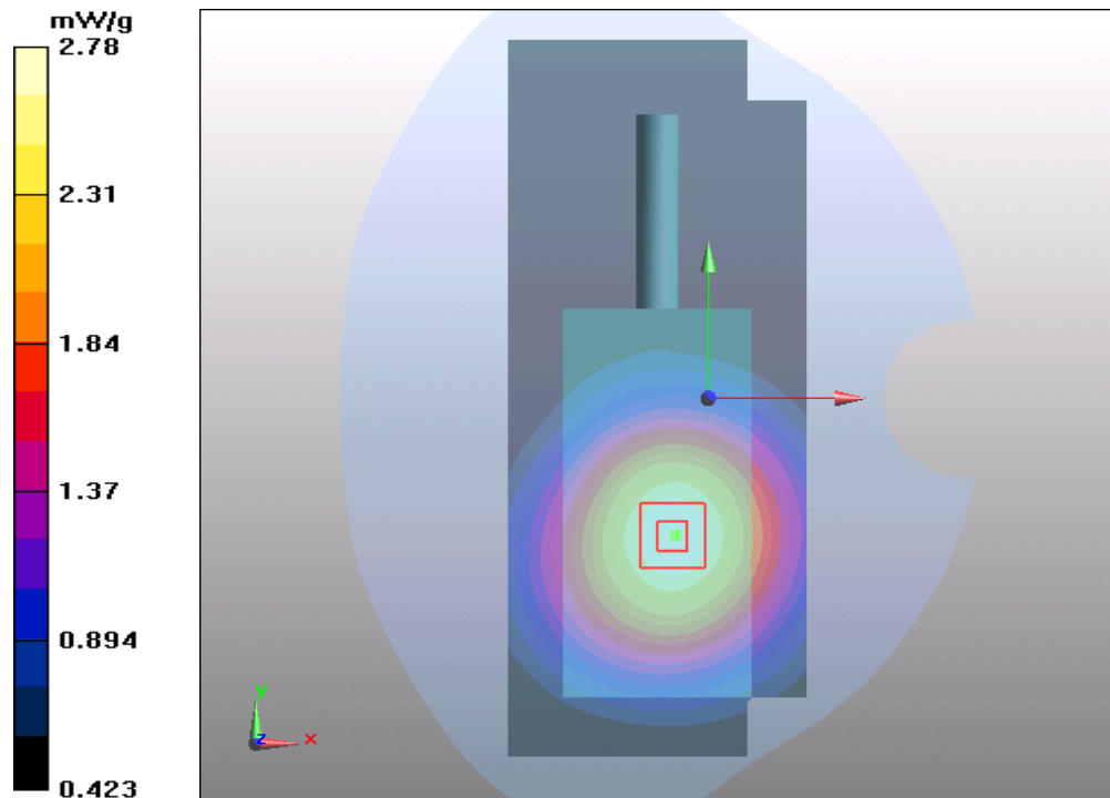
Figure 12 Face Held, Front towards Phantom 869MHz (25 KHz Channel Spacing)
