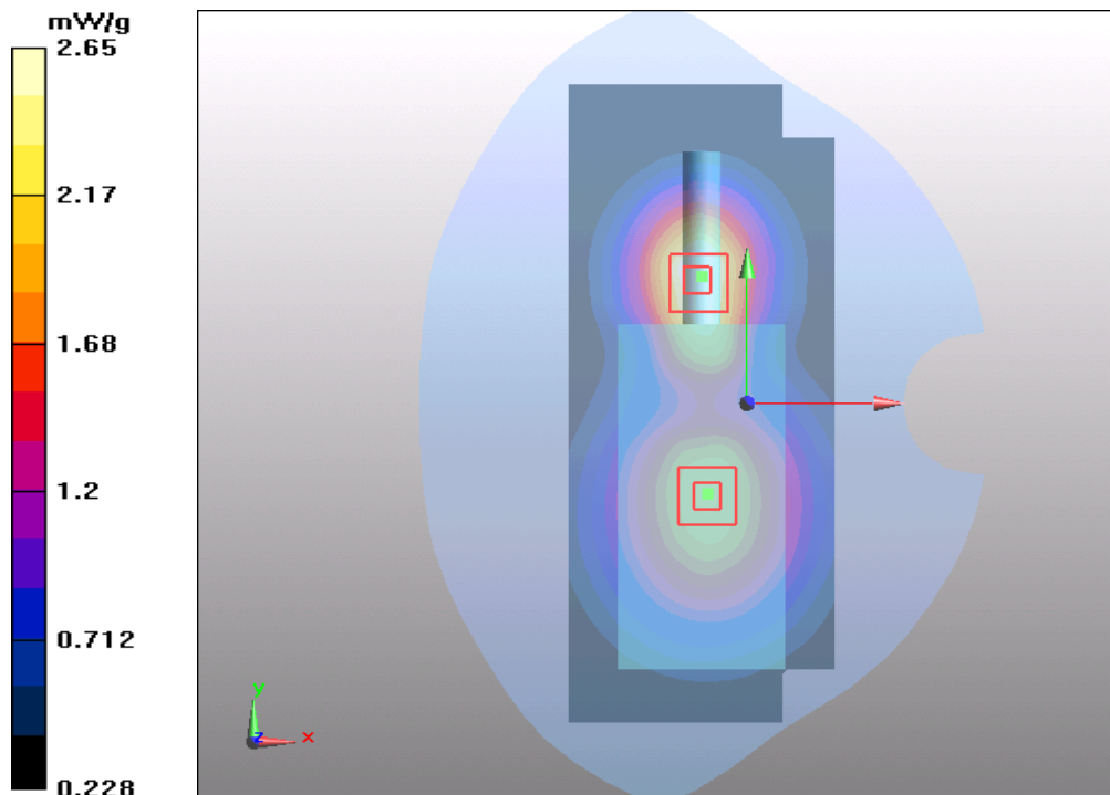
Figure 15 Body-Worn, Front towards Ground 862MHz (25 KHz Channel Spacing)
