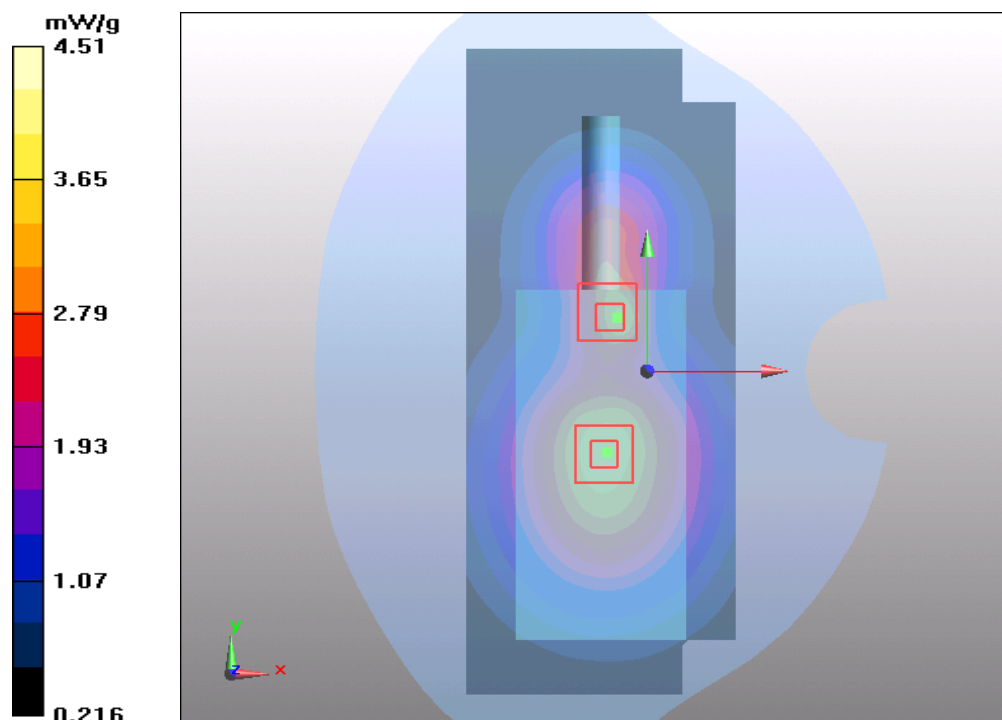
Figure 14 Body-Worn, Front towards Ground 824MHz (25 KHz Channel Spacing)
