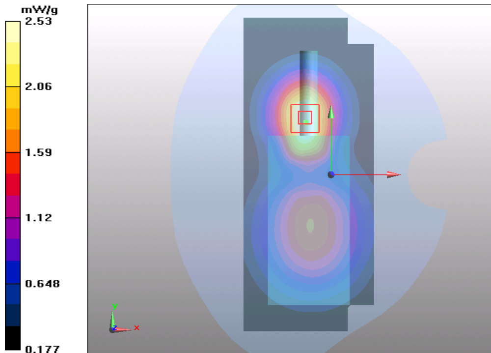
Figure 16 Body-Worn, Front towards Ground 869MHz (25 KHz Channel Spacing)
