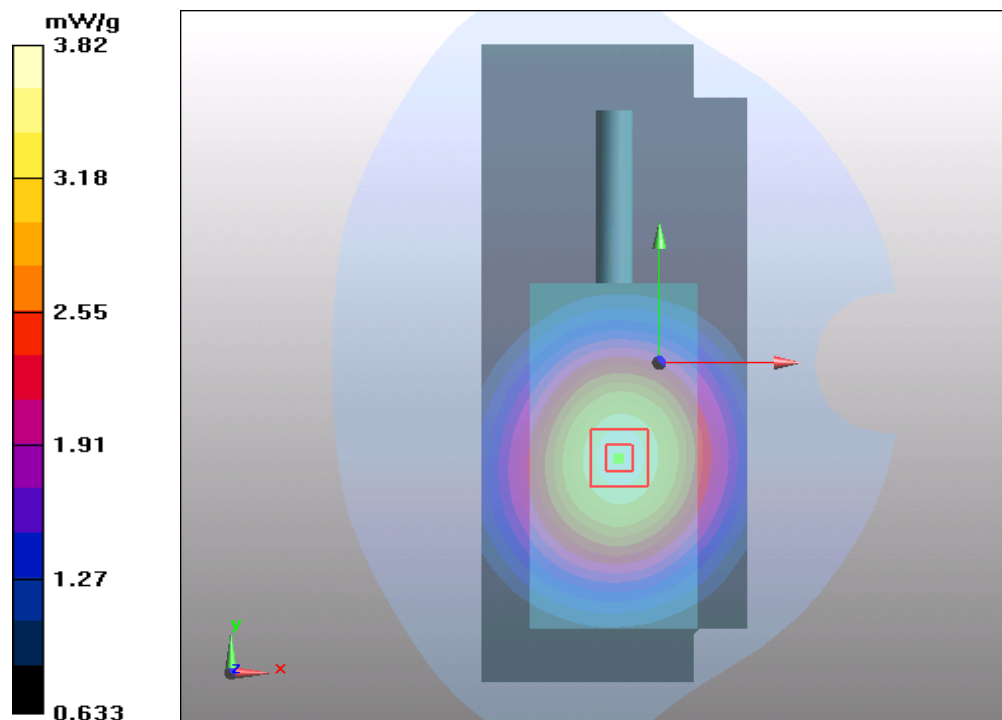
Figure 9 Face Held, Front towards Phantom 817MHz (25 KHz Channel Spacing)
