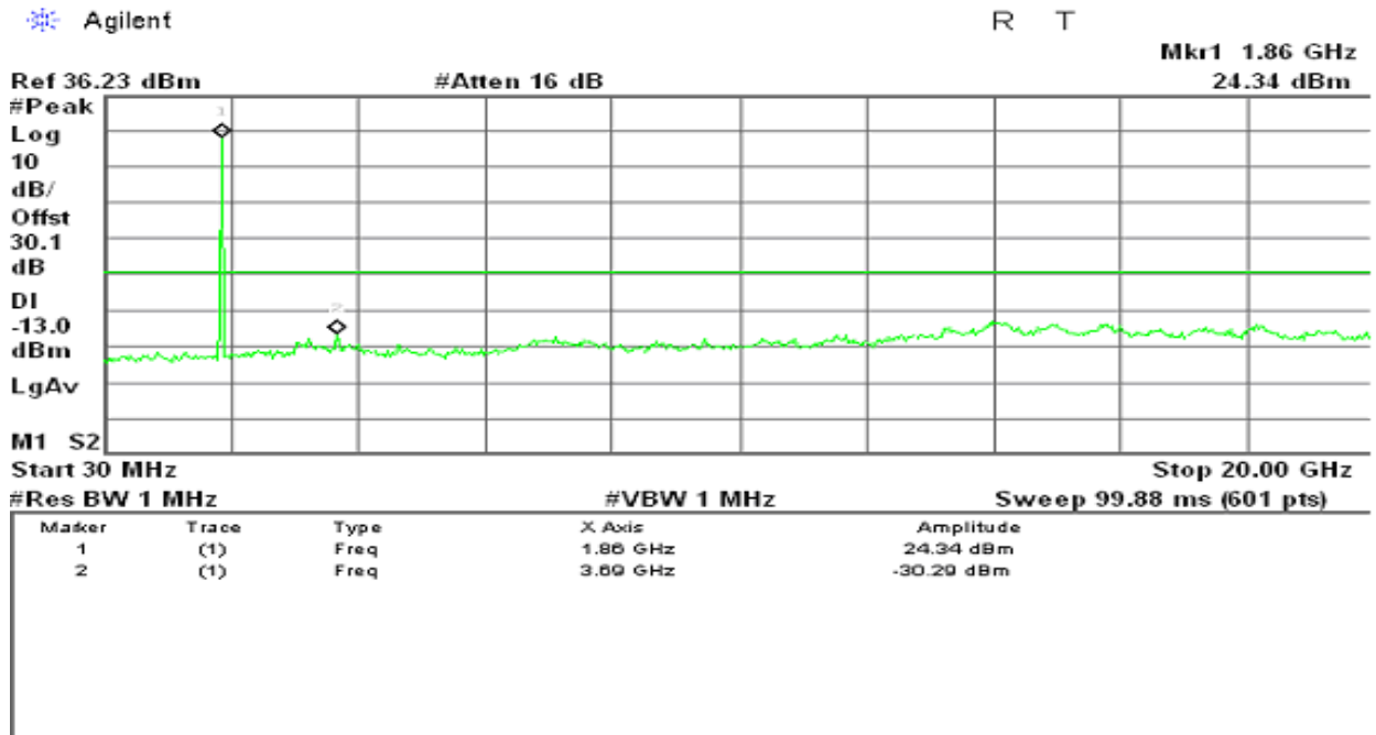
Figure 13-2: Out of Band emission at antenna terminals – WCDMA CH Mid
