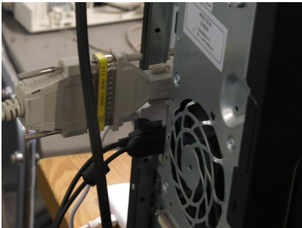
Conducted Emission back view
