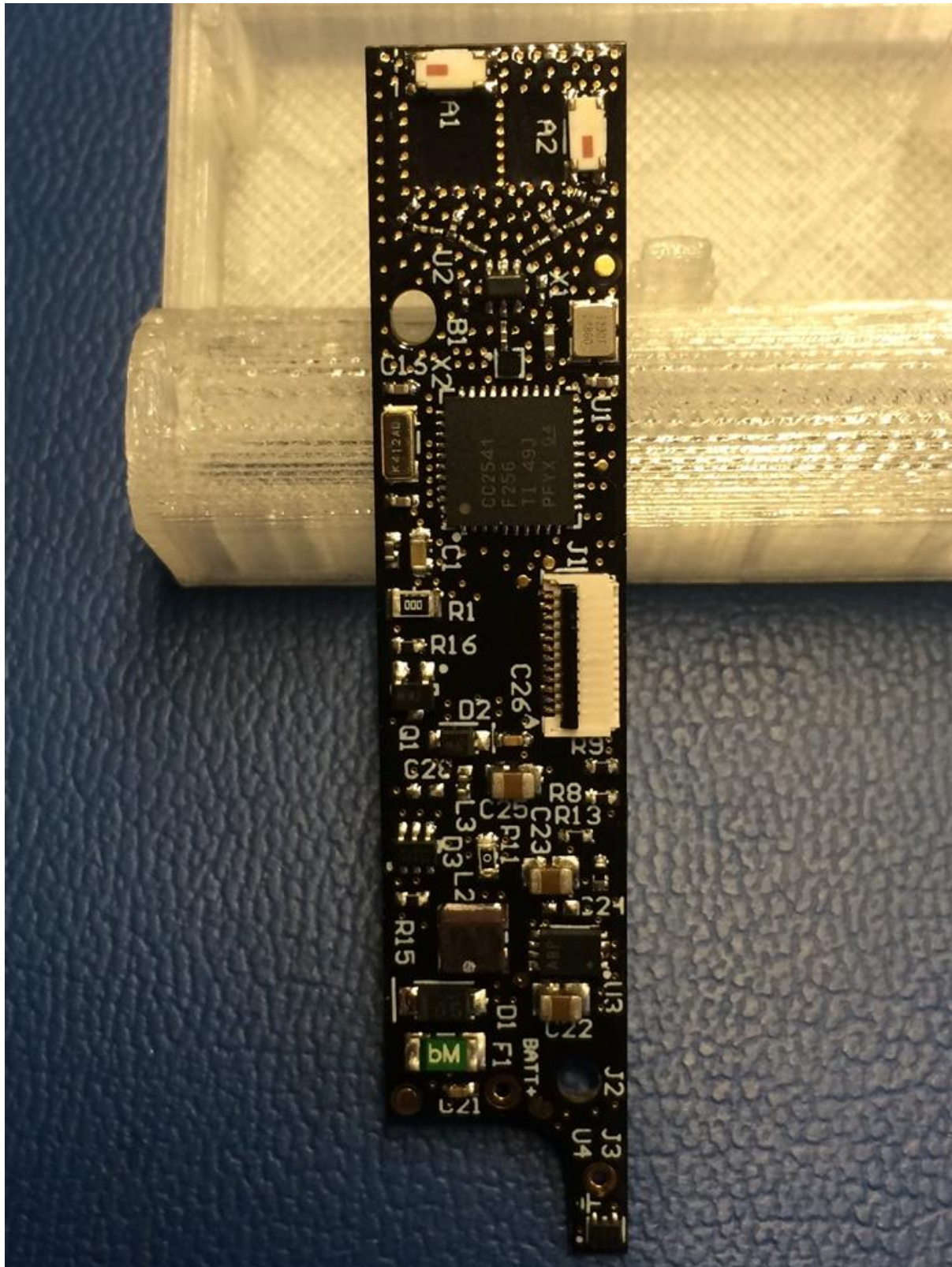
Fig. 3: TTV2-Belt Belt top of PCBA
