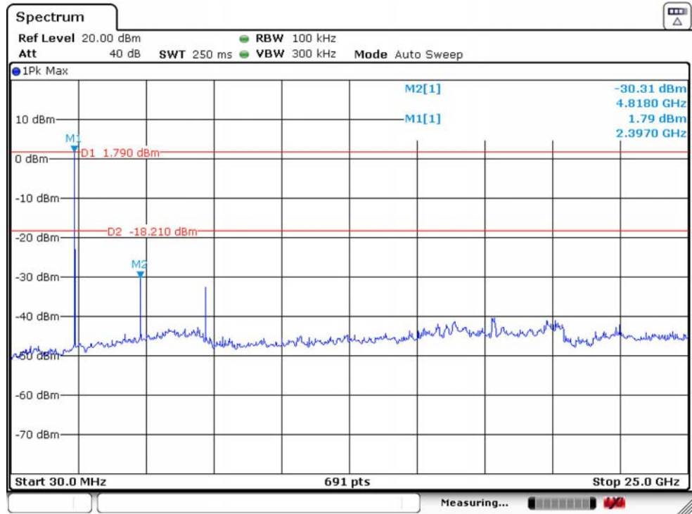
GFSK 2402 MHz
