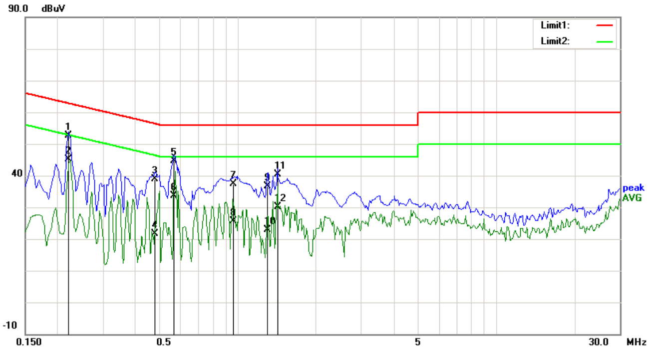
Phase Natural Plot at 240V AC, 60Hz
