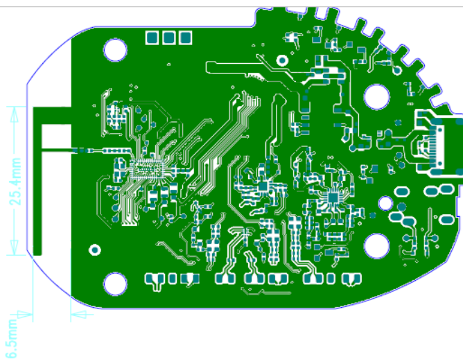
Antenna Dimensions
