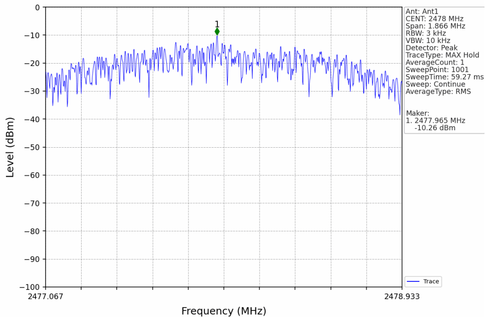
2M_HCH_2478MHz_Ant1_NTNV
