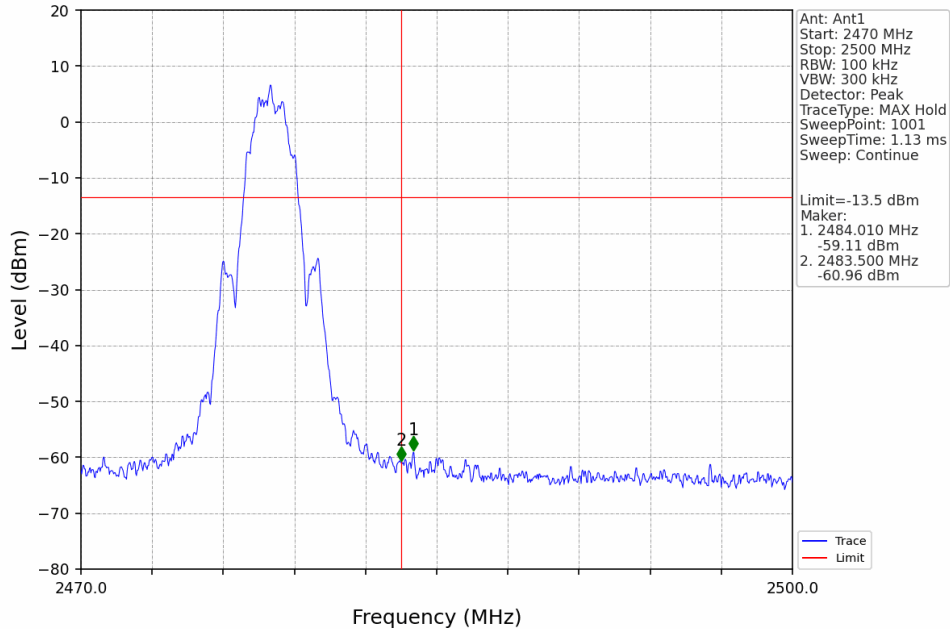
2M_HCH_2478MHz_Ant1_NTNV
