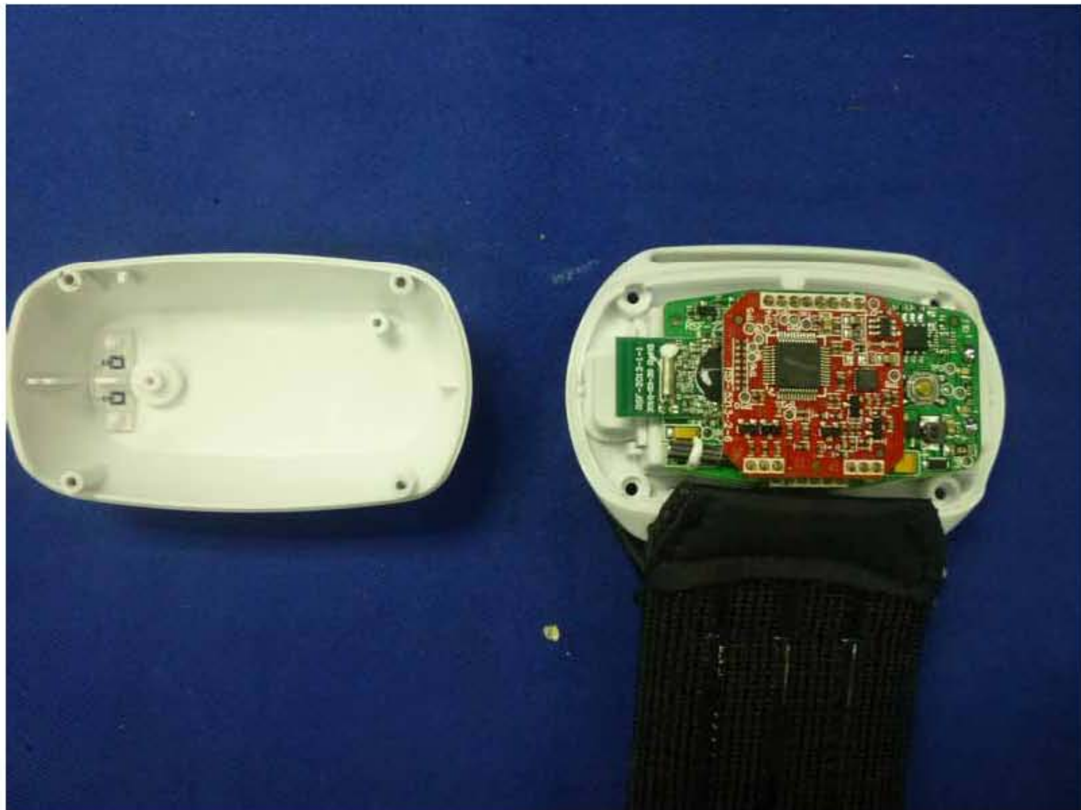
Figure 2 Inside of the EUT
