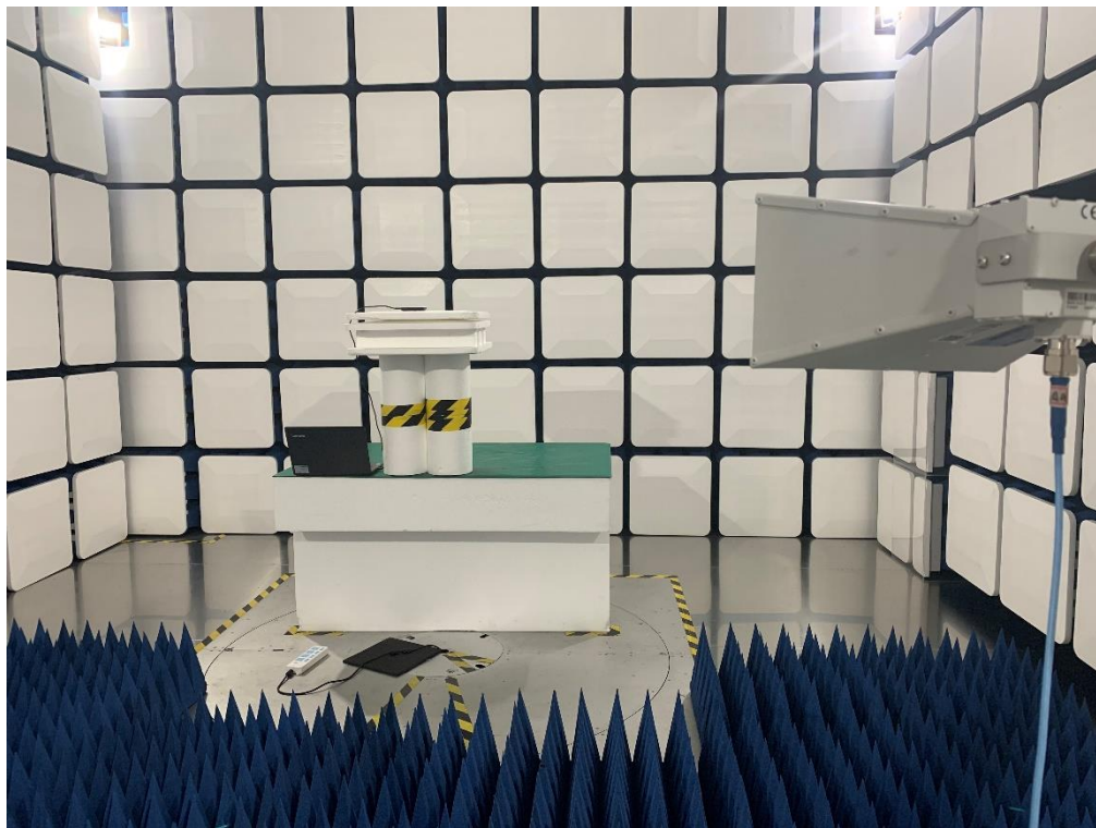
Above 1GHz-WIFI
