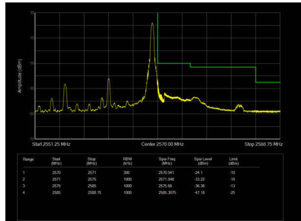
LTE Band 7 16QAM 15MHz CH-High, 1 RB
