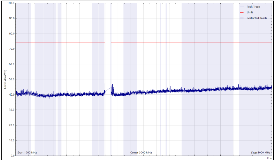
Figure 4 - 2462 MHz (CH11), 802.11b, 1 GHz to 5 GHz, Horizontal (Peak)
