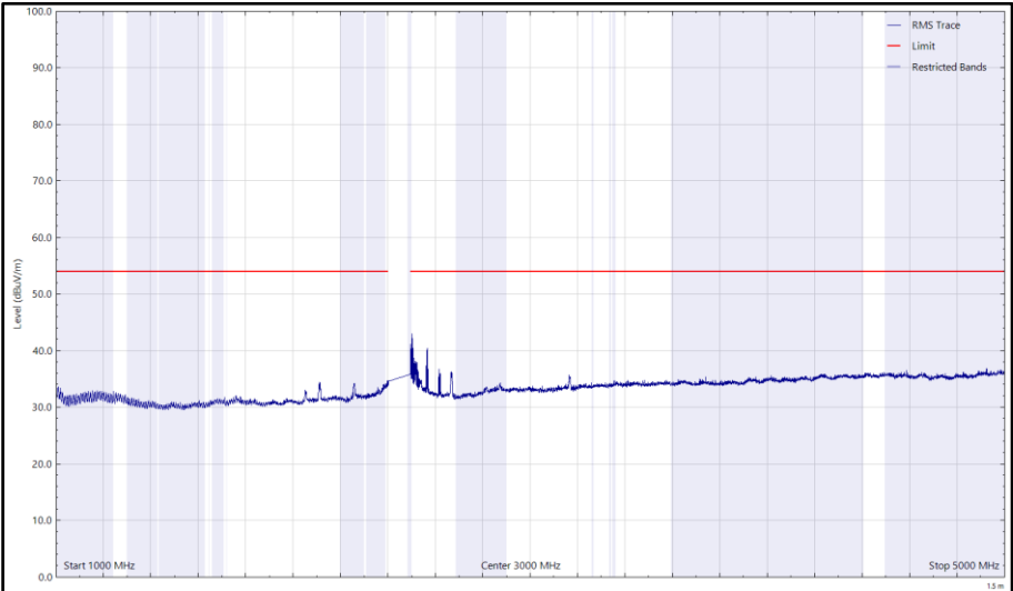
Figure 7 - 2462 MHz (CH11), 802.11b, 1 GHz to 5 GHz, Vertical (rms)
