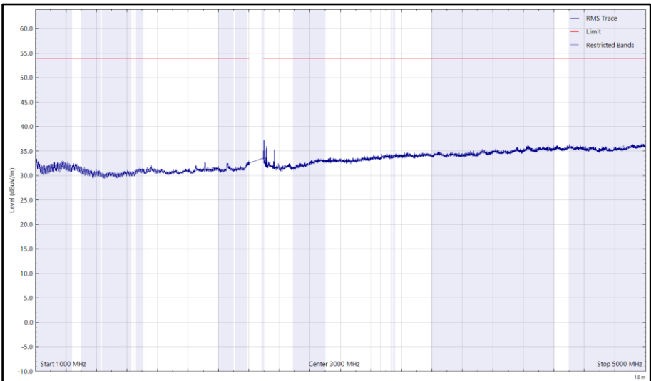
Figure 3 - 2462 MHz (CH11), 802.11b, 1 GHz to 5 GHz, Horizontal (rms)
