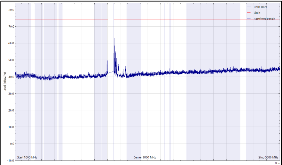
Figure 6 - 2462 MHz (CH11), 802.11b, 1 GHz to 5 GHz, Vertical (Peak)
