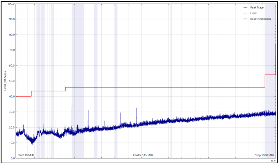
Figure 2 - 2462 MHz (CH11), 802.11b, 30 MHz to 1 GHz, Horizontal (Peak)
