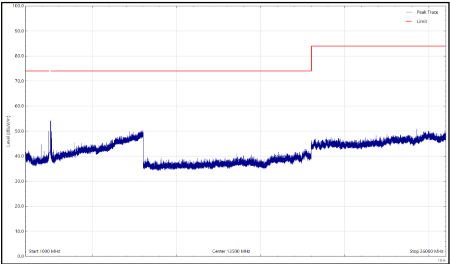
Figure 6 - 2462 MHz (CH11), 802.11b, 1 GHz to 26 GHz, Vertical (Peak)
