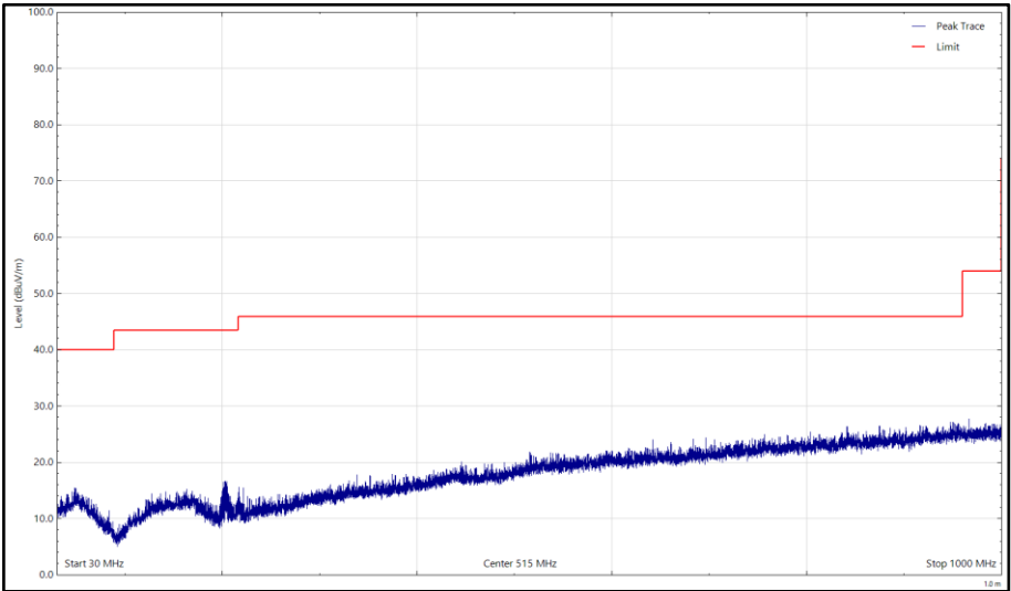
Figure 5 - 2462 MHz (CH11), 802.11b, 30 MHz to 1 GHz, Vertical (Peak)
