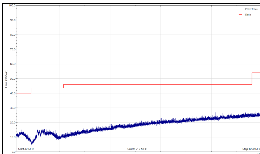
Figure 2 - 2462 MHz (CH11), 802.11b, 30 MHz to 1 GHz, Horizontal (Peak)
