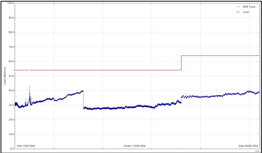
Figure 7 - 2462 MHz (CH11), 802.11b, 1 GHz to 26 GHz, Vertical (rms)
