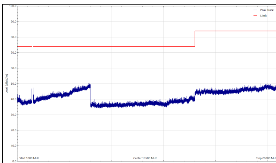
Figure 3 - 2462 MHz (CH11), 802.11b, 1 GHz to 26 GHz, Horizontal (Peak)
