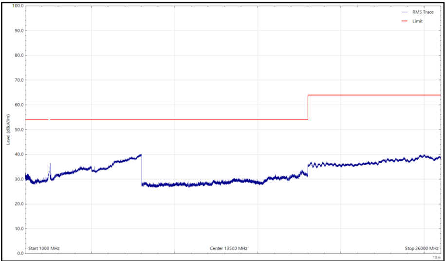
Figure 4 - 2462 MHz (CH11), 802.11b, 1 GHz to 26 GHz, Horizontal (rms)
