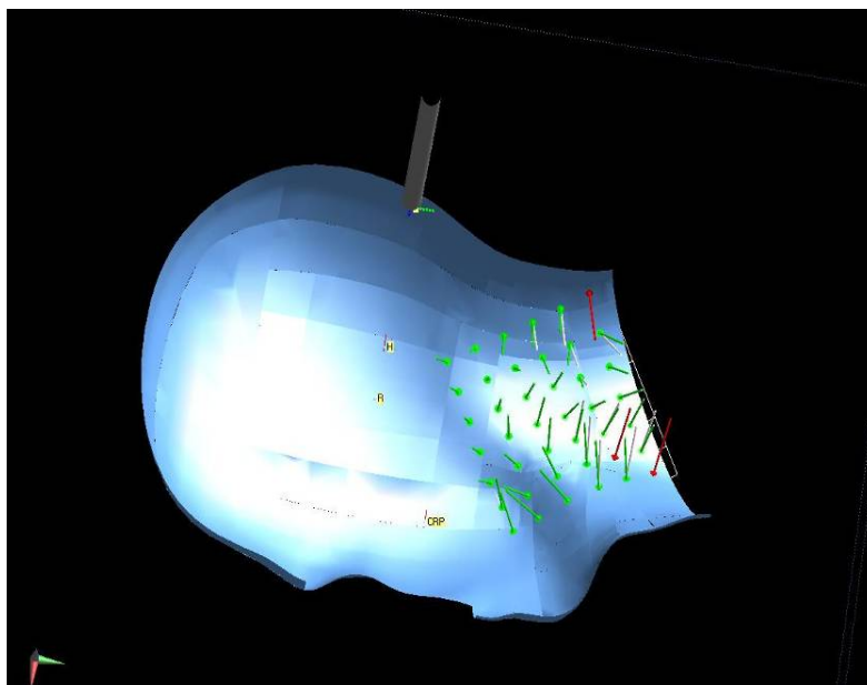
Probe Trajectories Plot (Position B)
