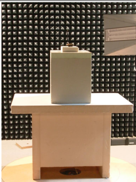
Figure 10: Measurement set-up for radiated measurement > 1 GHz acc. to following sections of the report 1114-11-EE-11-PB001: 4.4.4 and 4.5.2
