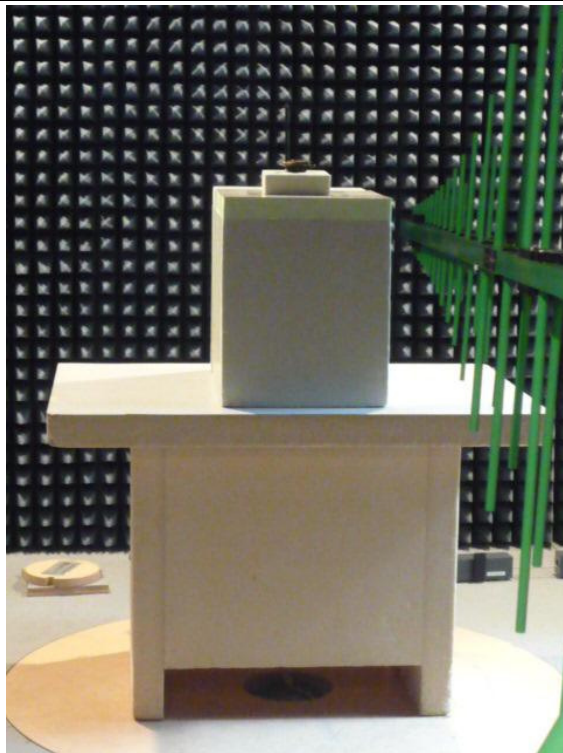
Figure 9: Measurement set-up for radiated measurement > 30 MHz and < 1 GHz acc. to following sections of the report 1114-11-EE-11-PB001: 4.4.2; 4.4.3 and 4.5.1
