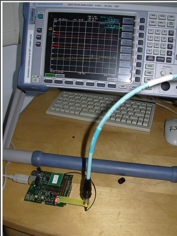
Figure 7: Measurement set-up for conducted measurement acc. to following sections of the report 1114-11-EE-11-PB001: 4.1.1; 4.1.2; 4.2; 4.3 and 4.4.5
