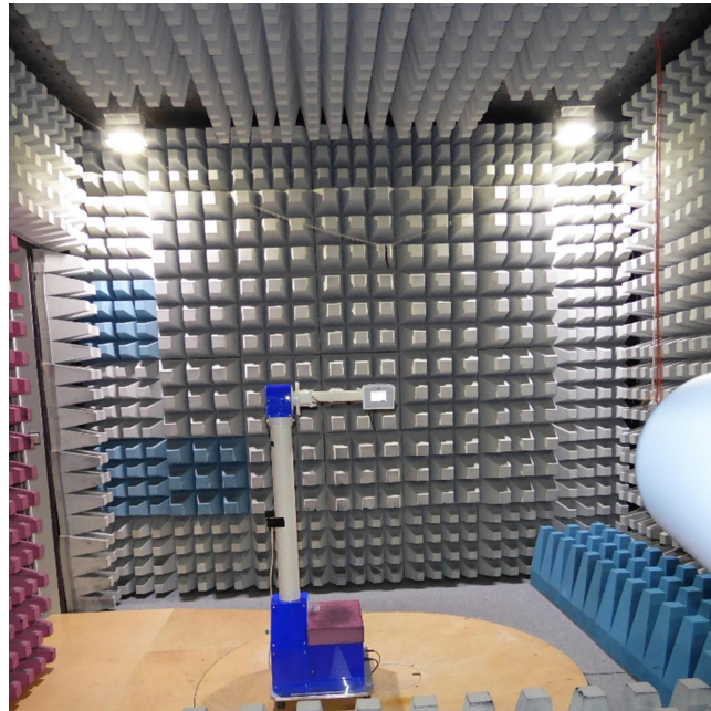
EUT on positioner Test setup fully anechoic chamber M20
