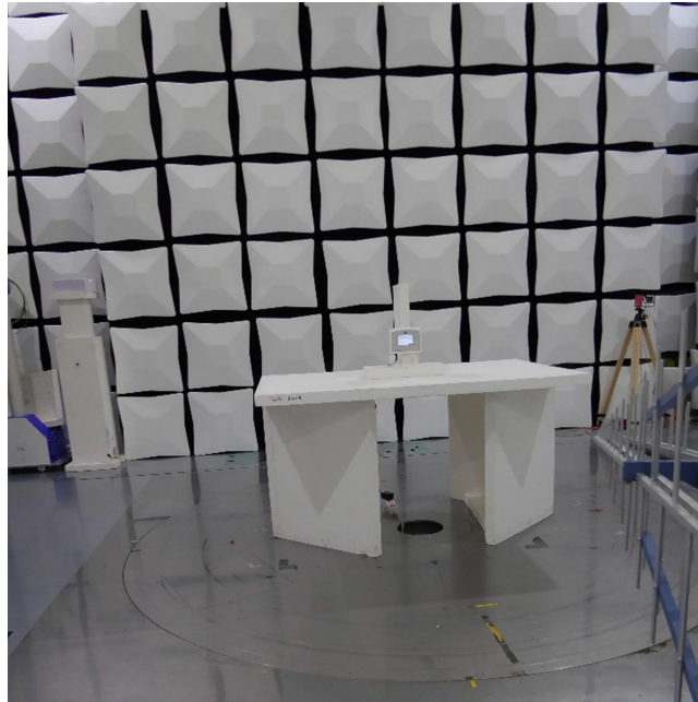
Test setup semi-anechoic chamber M276
