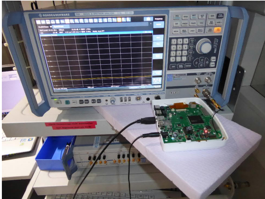
Test setup conducted @ antenna port
