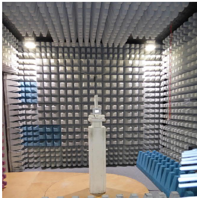
Test setup fully anechoic chamber M20
