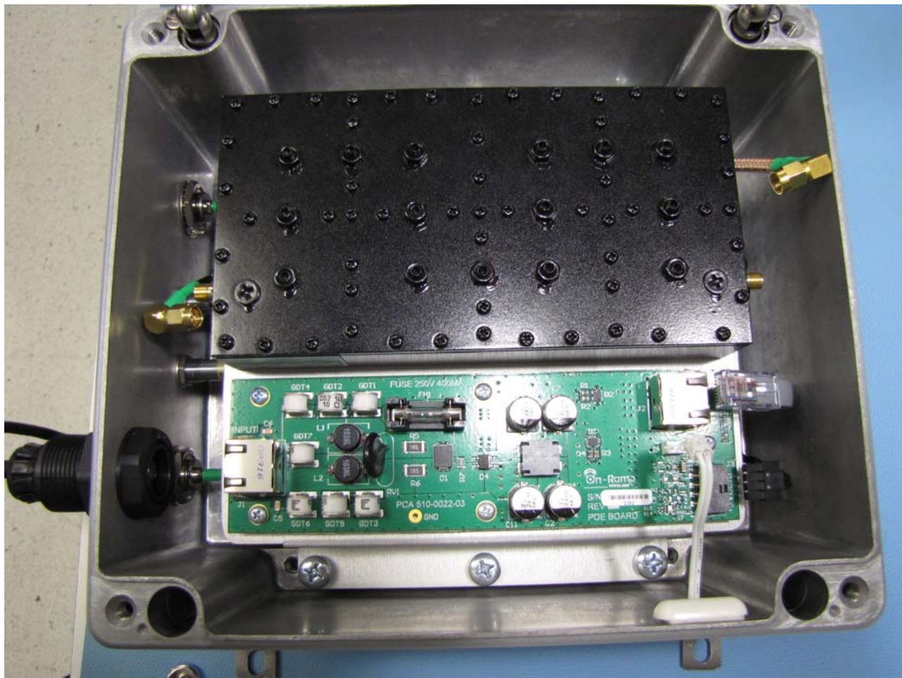
Cavity filter over main board.
