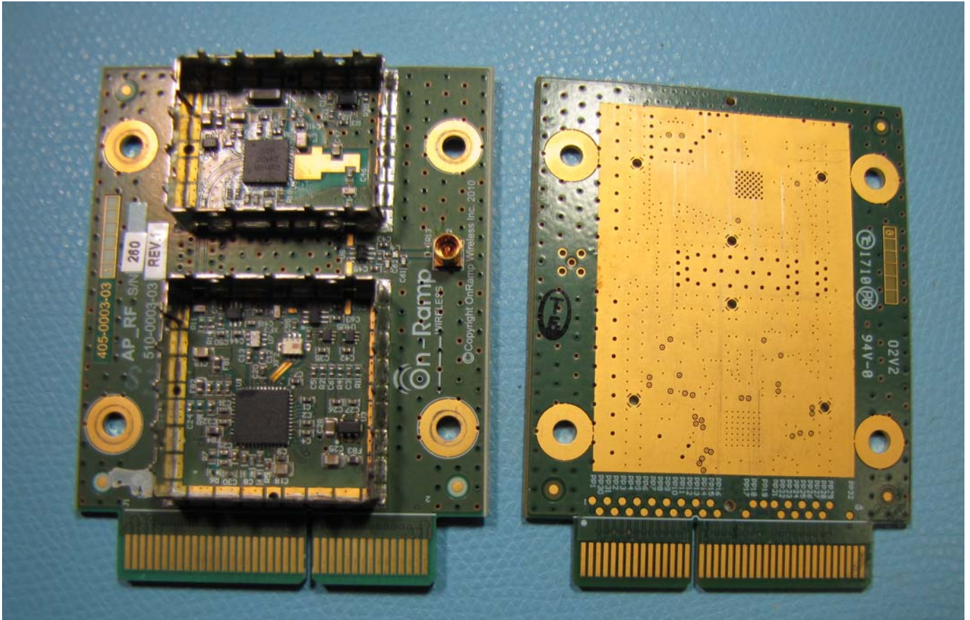
RF board with Shields Removed.
