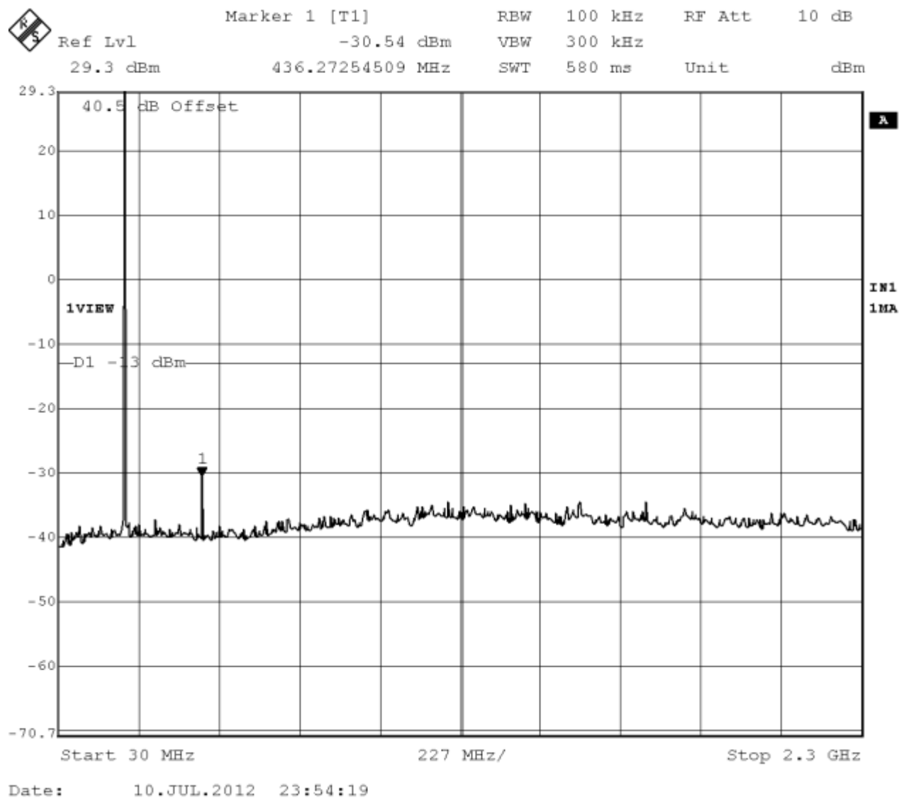
Figure 22: Out of Band Emissions Operating Channel 218.5 MHz, GMSK
