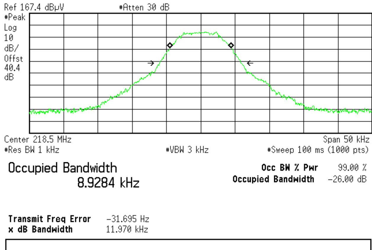
Figure 13: Occupied Bandwidth at— Operating Channel 218.5 MHz GMSK
