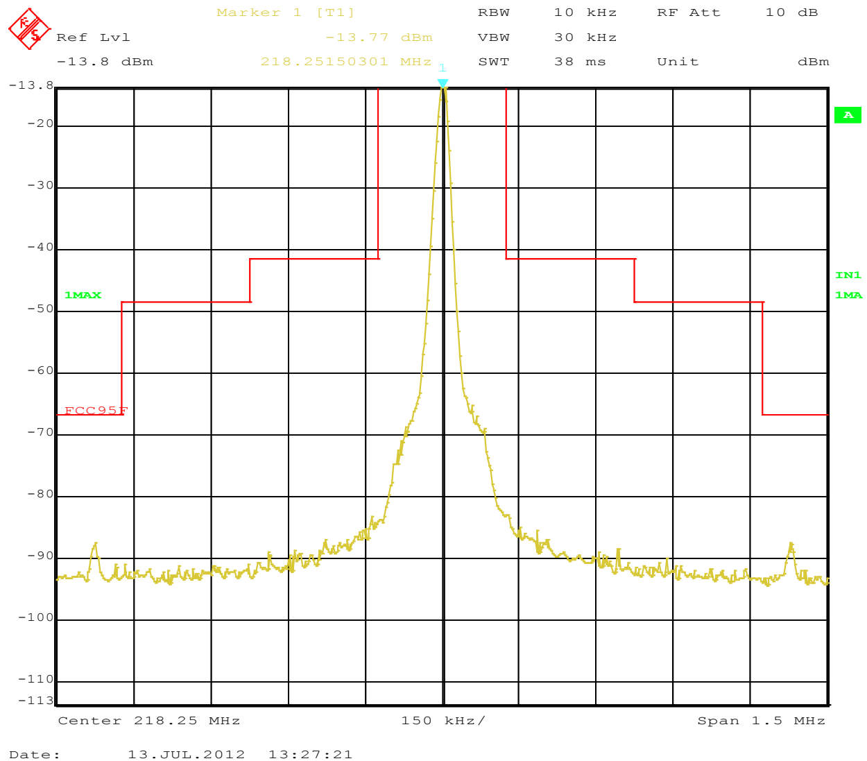
Figure 20: Emission mask Requirement at Operating Channel 218.25 MHz, 16 QPSK
