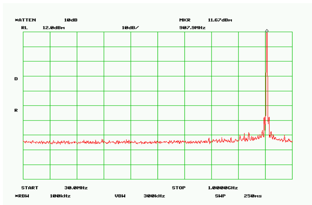
Plot 10 – Low Band
