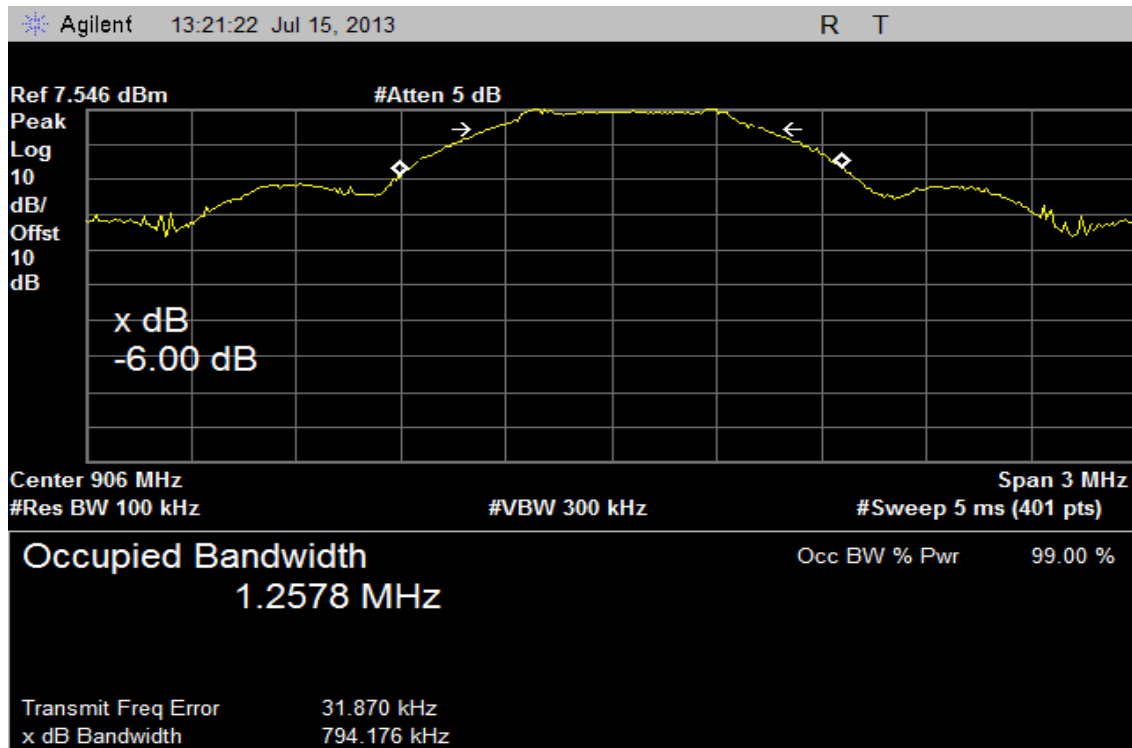
Plot 4 – Lowest Channel – 6dB BW (Random Data Set-prbs)
