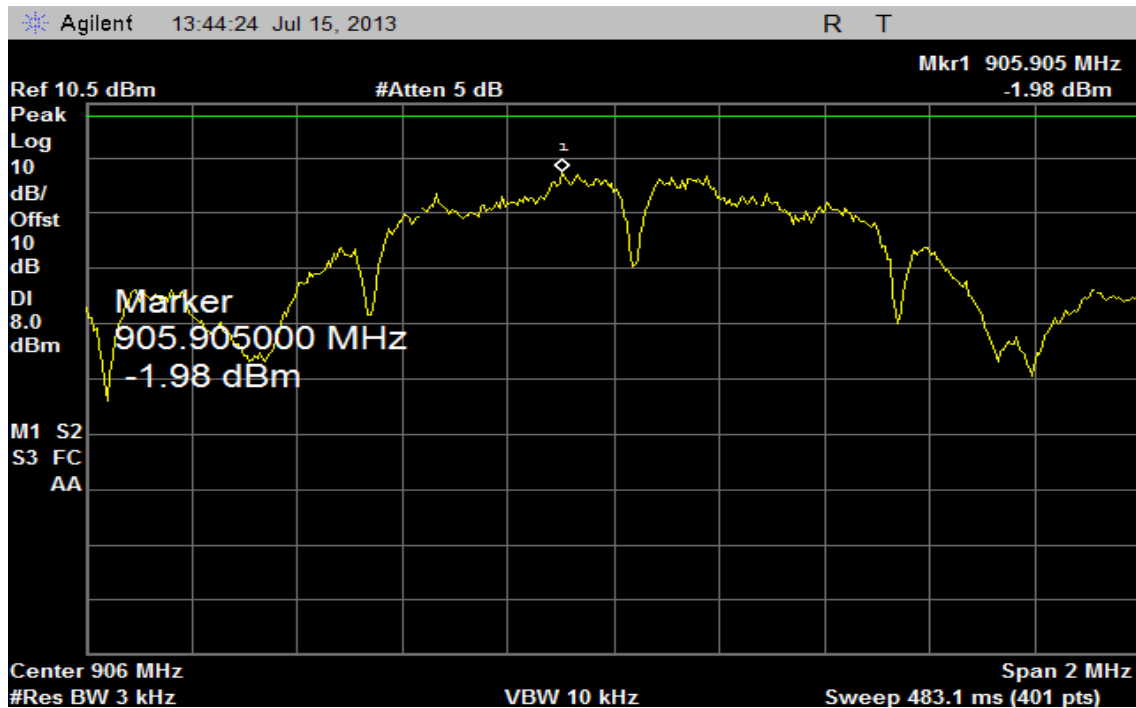
Plot 18 – Power Spectral Density – Lowest Channel
