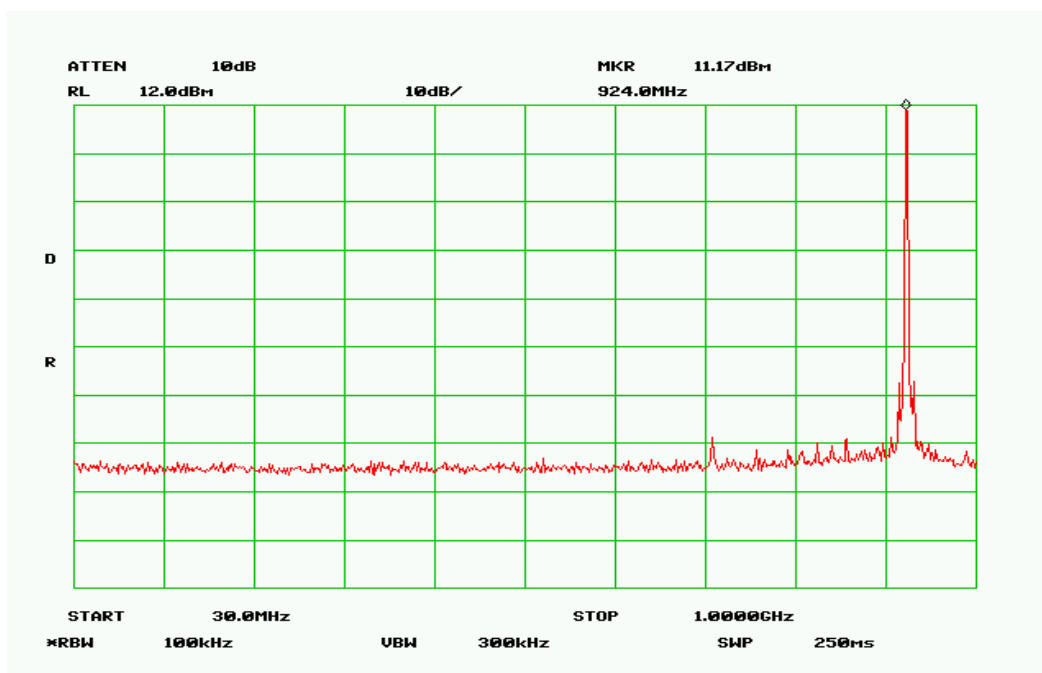
Plot 14 – High Band
