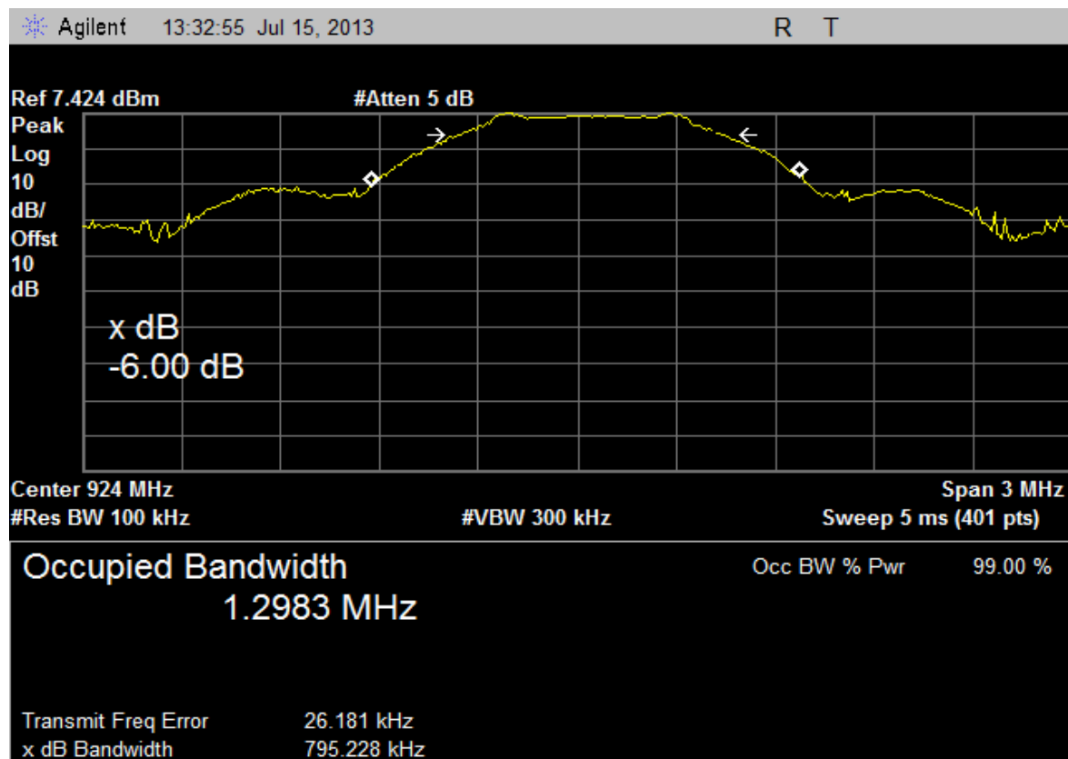
Plot 6 – Highest Channel – 6dB BW (Random Data Set - prbs)
