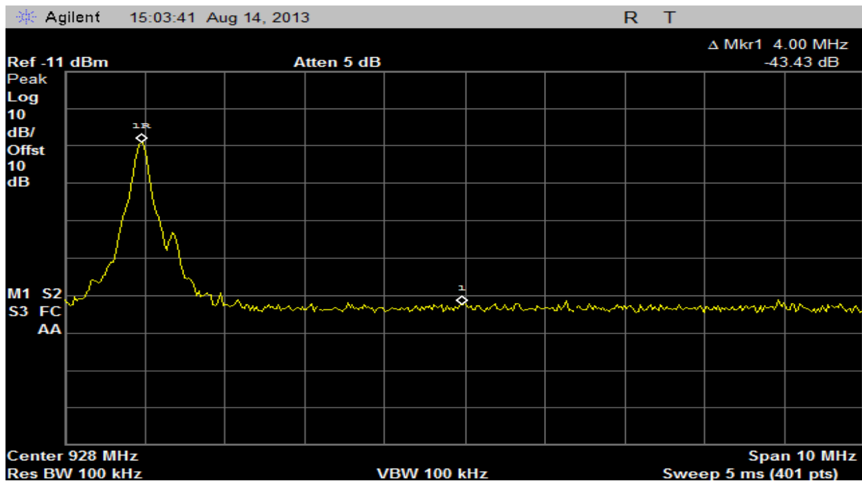
Plot 17 – Band Edge High Channel
