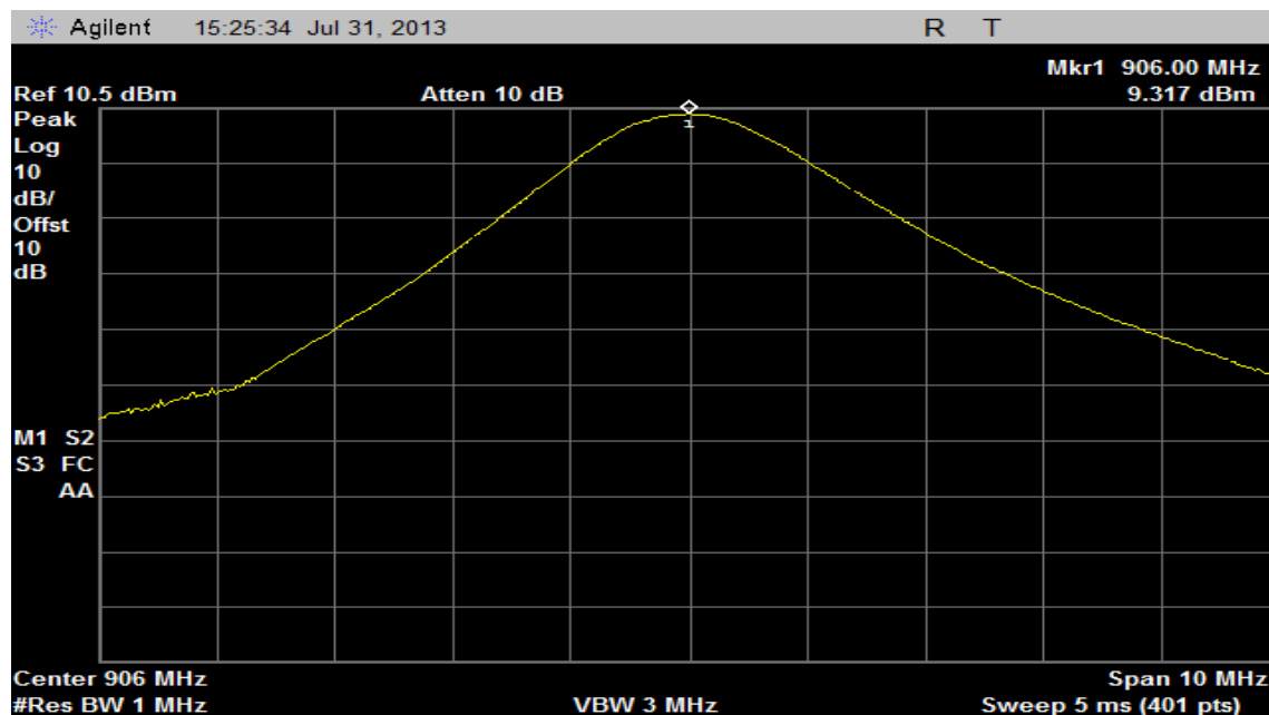
Plot 7 – Output Power – Low Channel
