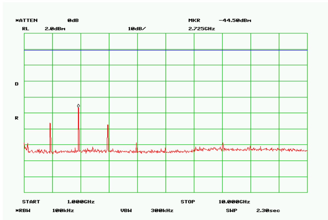
Plot 13 – Mid Band
