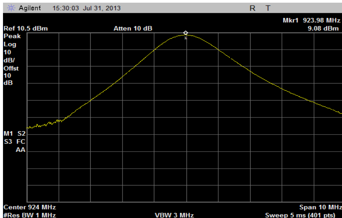
Plot 9 – Output Power – High
