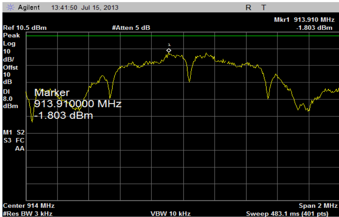
Plot 19 – Power Spectral Density – Middle Channel
