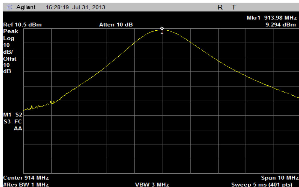
Plot 8 – Output Power – Mid Channel
