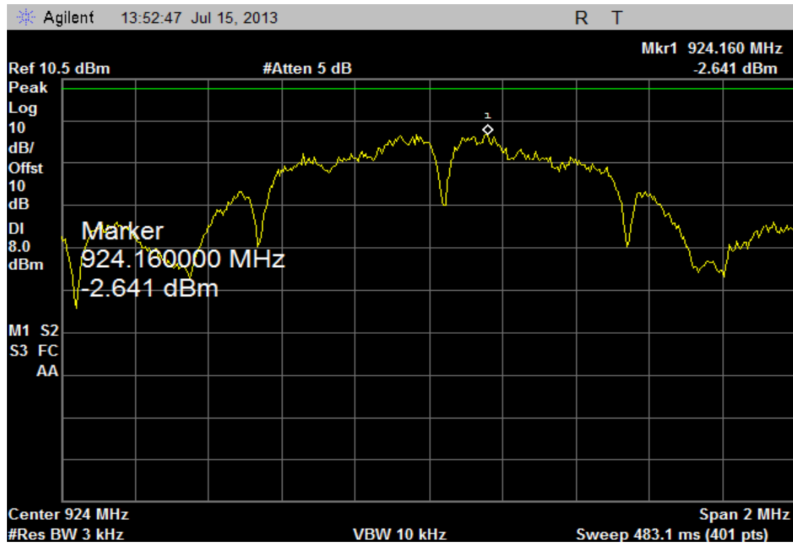
Plot 20 – Power Spectral Density – Highest Channel
