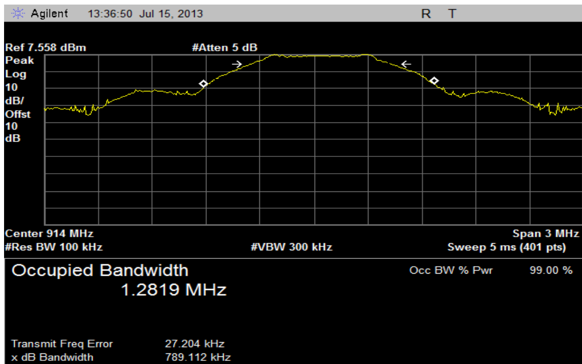
Plot 5 – Middle Channel – 6dB BW (Random Data Set-prbs)
