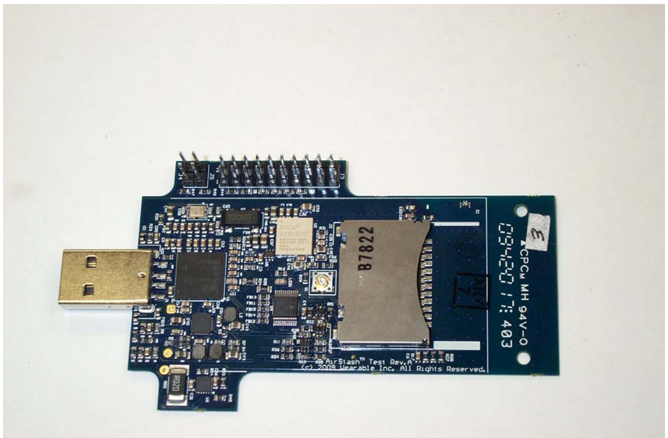
Component Side of USB powered EUT
