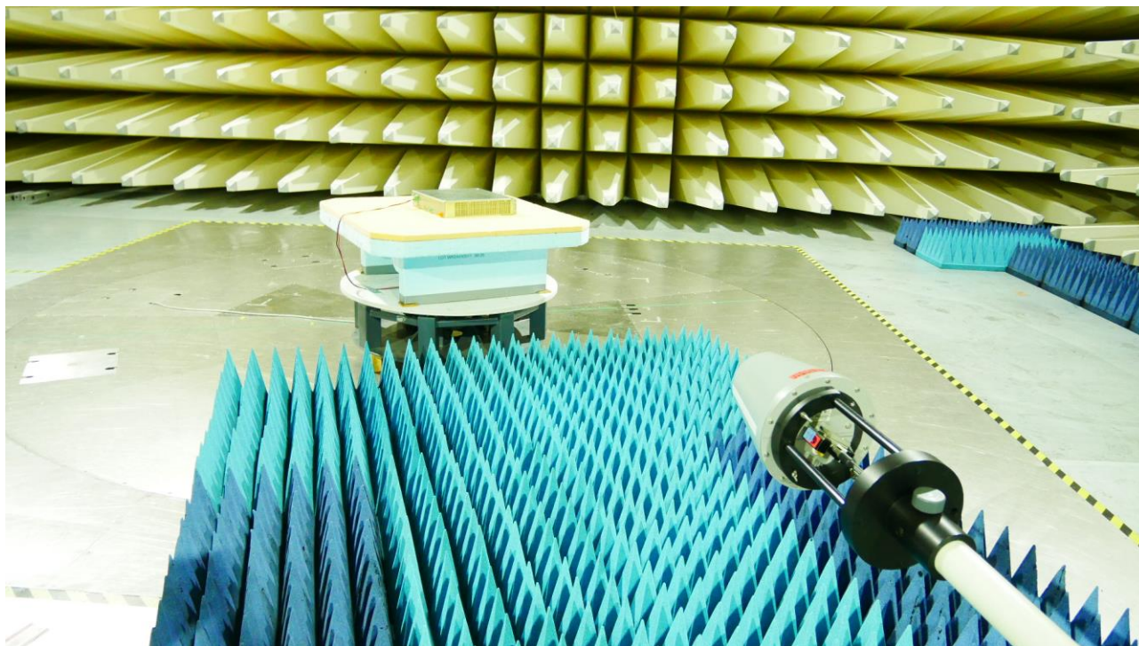
Test setup for radiated emissions in the frequency range 1 – 6 GHz
