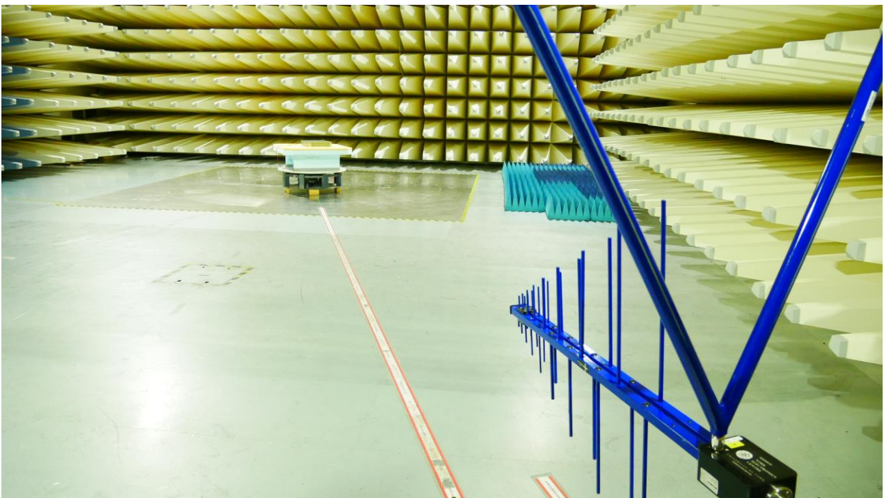
Test setup for radiated emissions in the frequency range 30 – 1000 MHz
