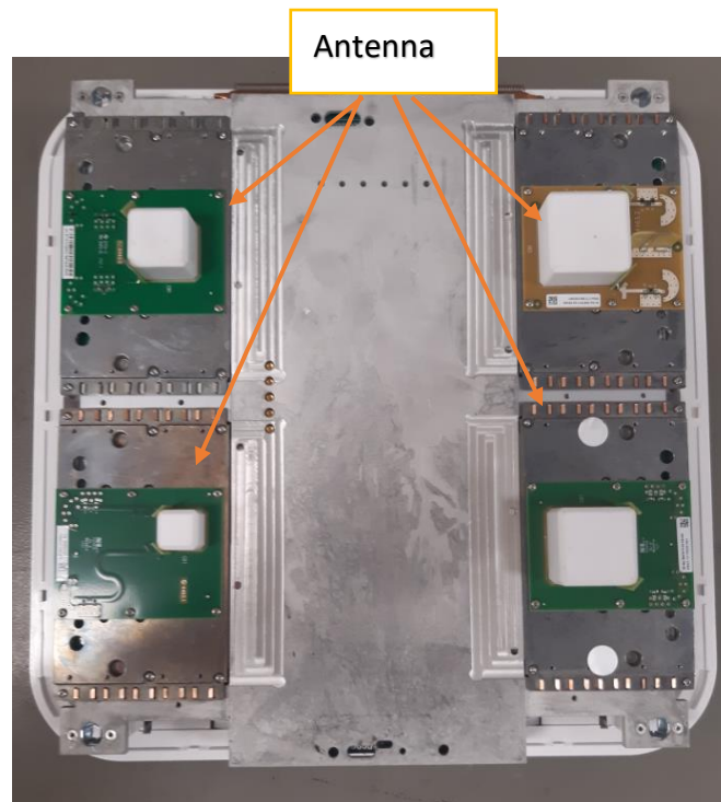
UAP 2 without upper cover
