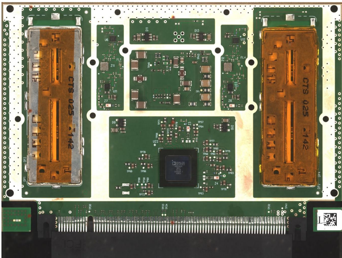
RM 19 – 7843225-03 – BOTTOM View
