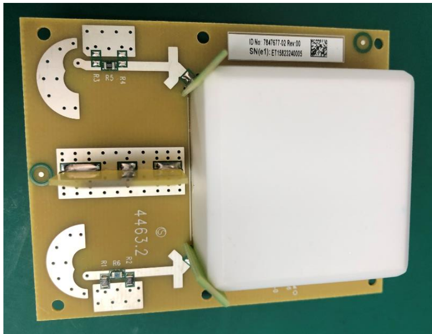
Antenna 17E – 7847677-02 – TOP View
