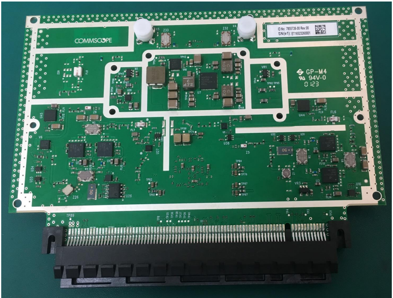
RM 37T – Assembled PCB 7855726-00- Internal picture
