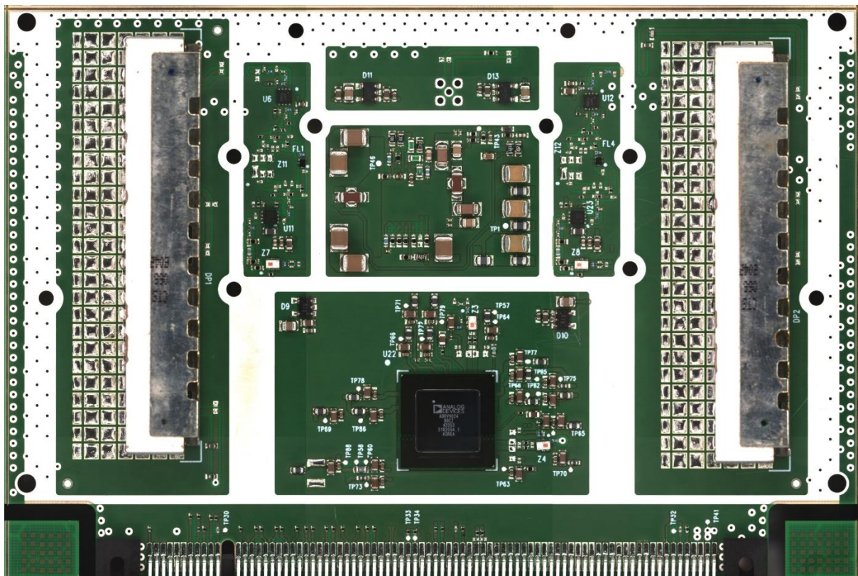
BOTTOM View
