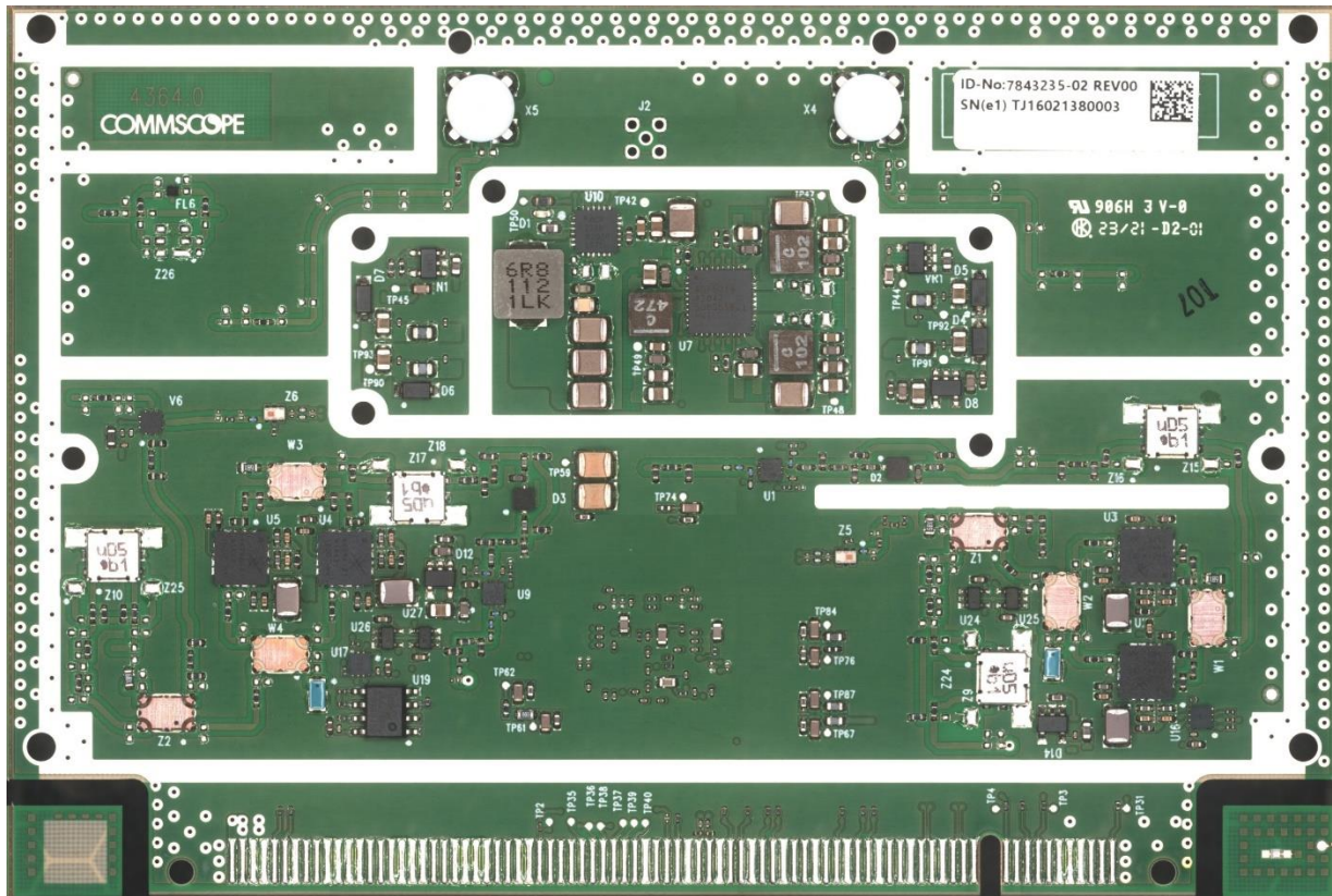
TOP View
