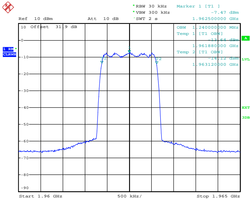
plot 6.3.1.3-#1 Occupied Bandwidth: §2.1049; Test results; Downlink; CDMA Output
