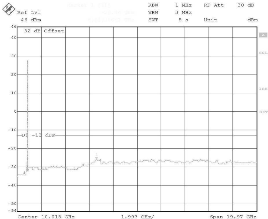
plot 7.3.1.9-#1 Spurious Emissions at Antenna Terminals: §24.238, §2.1051; Test results; Downlink; W-CDMA > 1MHz to band edge; carrier (1962,5MHz) notched
