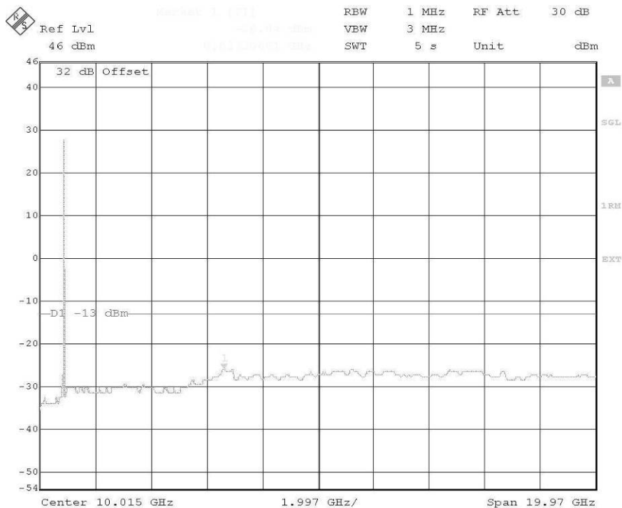
plot 7.3.1.8-#1 Spurious Emissions at Antenna Terminals: §24.238, §2.1051; Test results; Downlink; CDMA > 1MHz to band edge; carrier (1962,5MHz) notched
