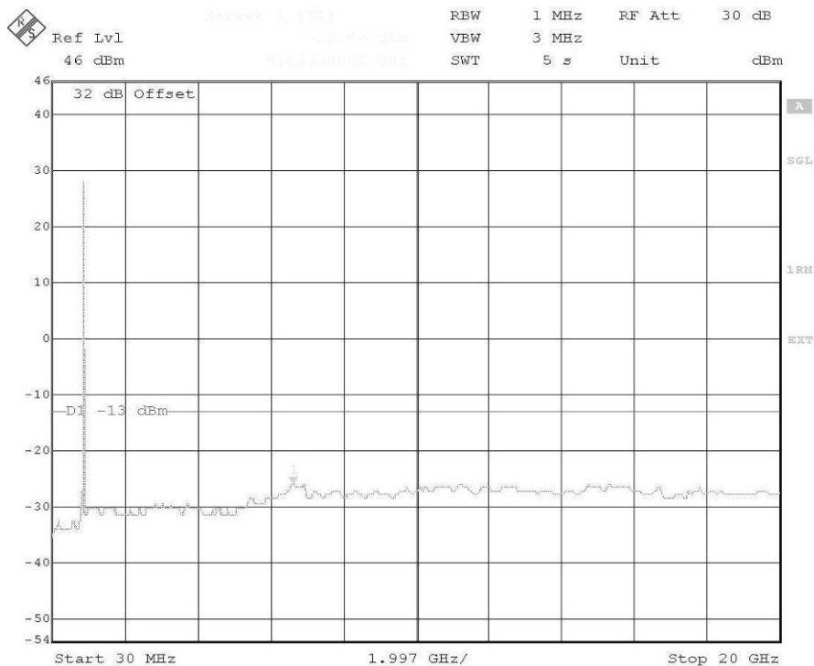
plot 7.3.1.6-#1 Spurious Emissions at Antenna Terminals: §24.238, §2.1051; Test results; Downlink; GSM > 1MHz to band edge; carrier (1962,5MHz) notched
