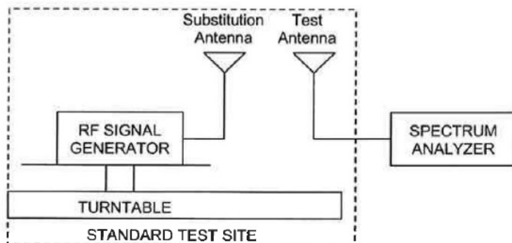
picture 8.3: Substitution method
