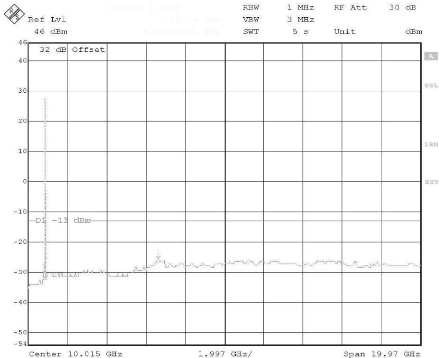
plot 7.3.1.10-#1 Spurious Emissions at Antenna Terminals: §24.238, §2.1051; Test results; Downlink; LTE > 1MHz to band edge; carrier (1962,5MHz) notched
