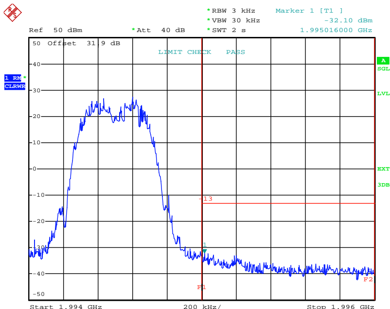
plot 7.3.1.2-#1 Spurious Emissions at Antenna Terminals: §24.238, §2.1051; Test results; Downlink; GSM-EDGE < 1MHz to band edge Lower Band Edge
