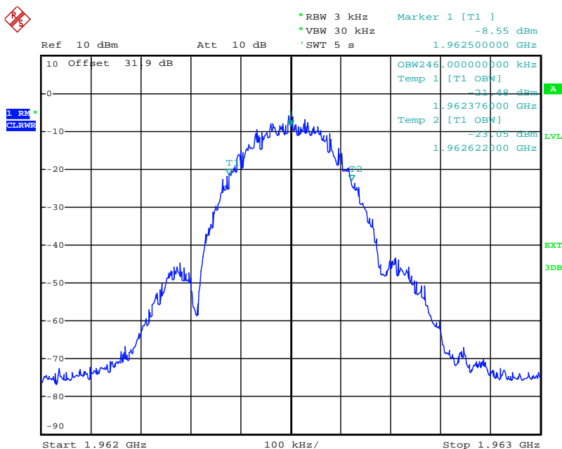
plot 6.3.1.2-#1 Occupied Bandwidth: §2.1049; Test results; Downlink; GSM-EDGE Output
