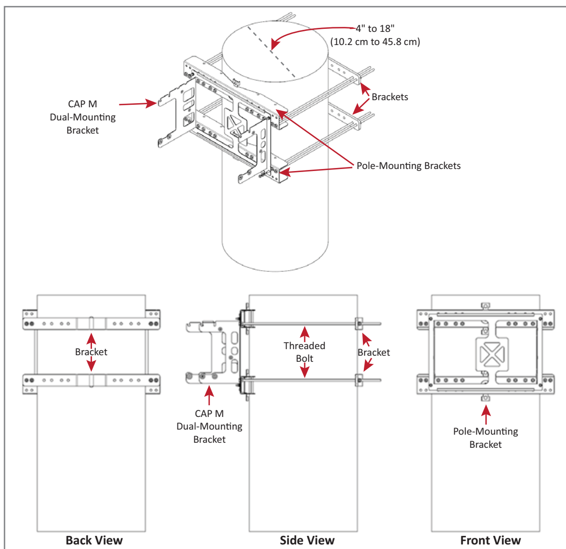
Figure 9. Installation Views of the CAP M Pole Mounting Kit for Up to 18" Poles (CommScope PN 7692096-XX)
