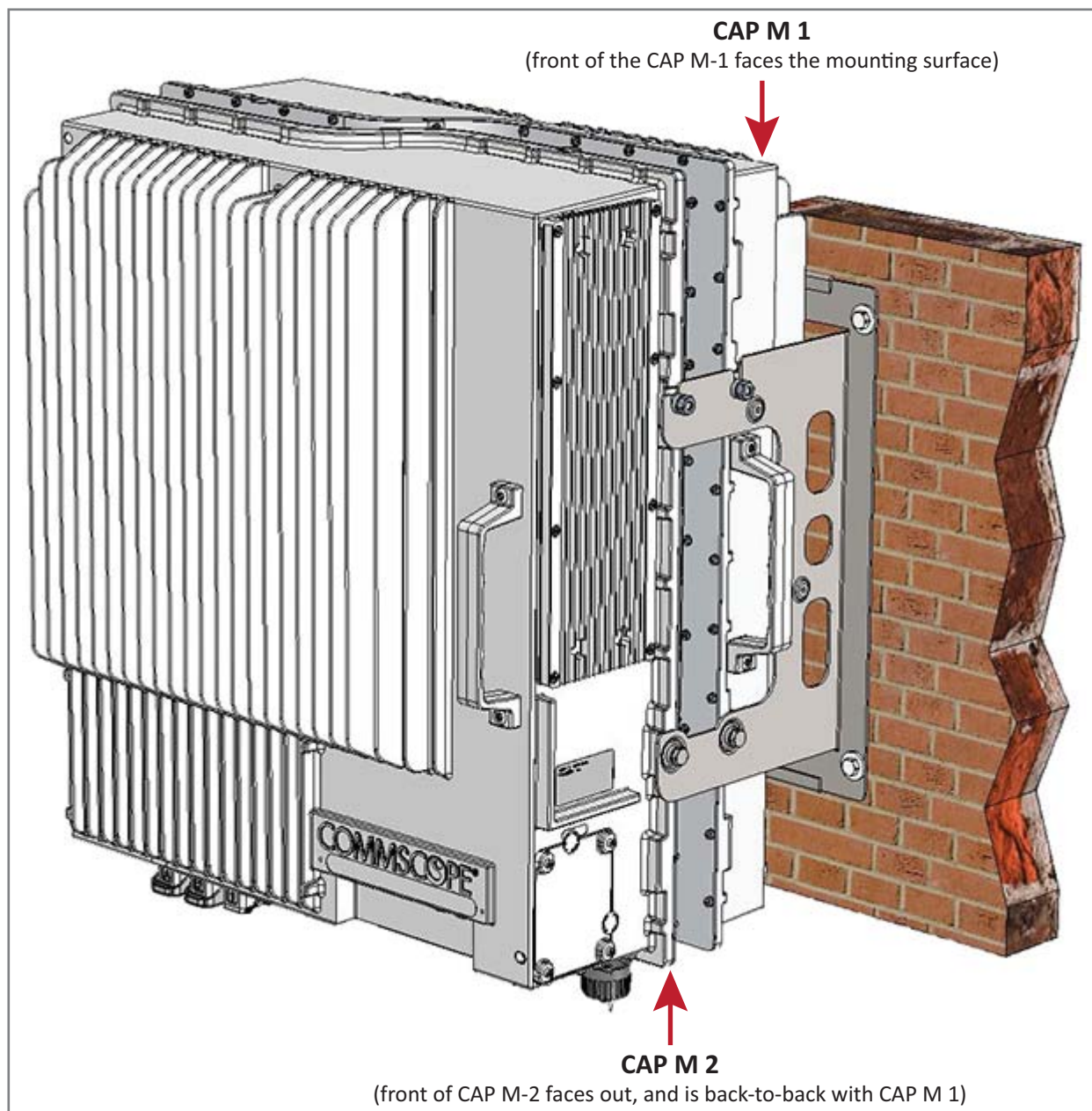
Figure 8. Two CAP Ms Back-to-Back in a Dual Mounting Bracket
