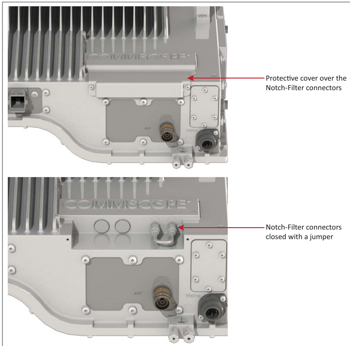
Figure 4. Notch-Filter Connector on the CAP M 7E/80-85/17E/19
