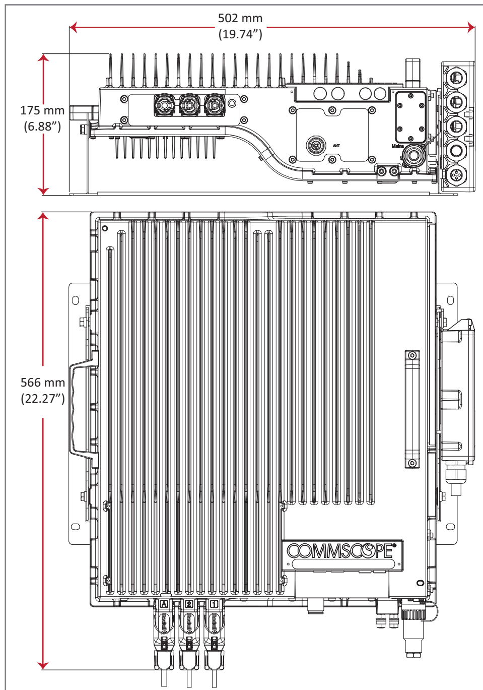
Figure 5. Mounting Dimensions with the Single Mounting Bracket
