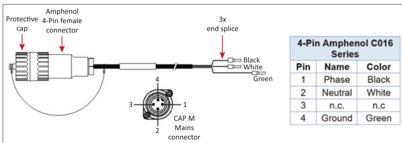
Figure 10. CAP M AC Power Cable
