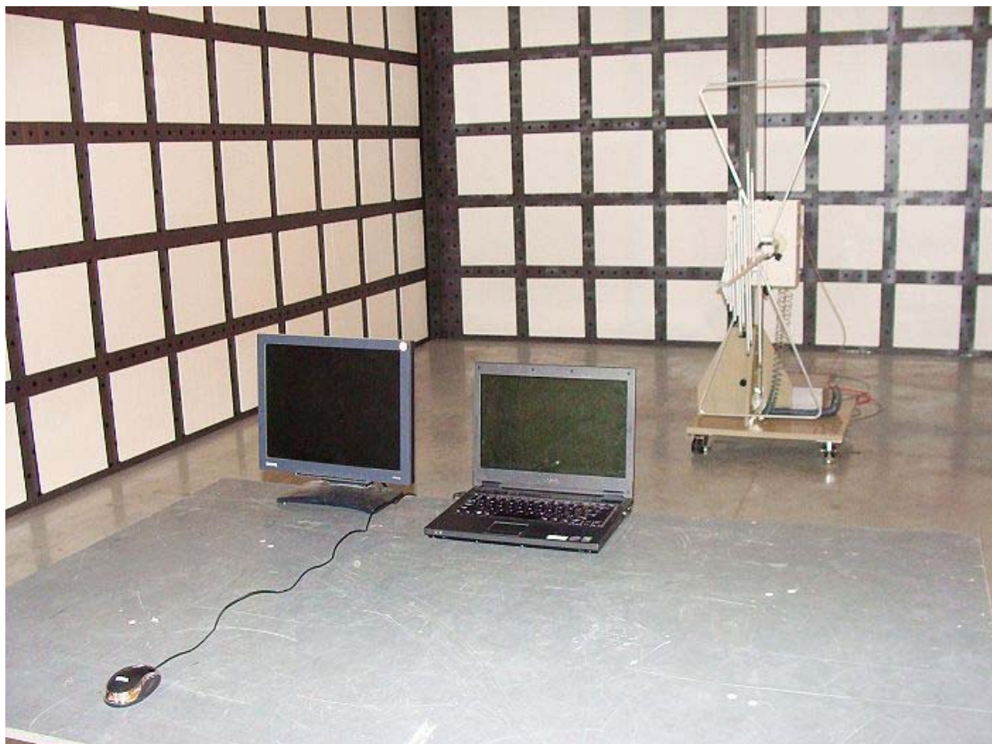
Radiated Emissions
