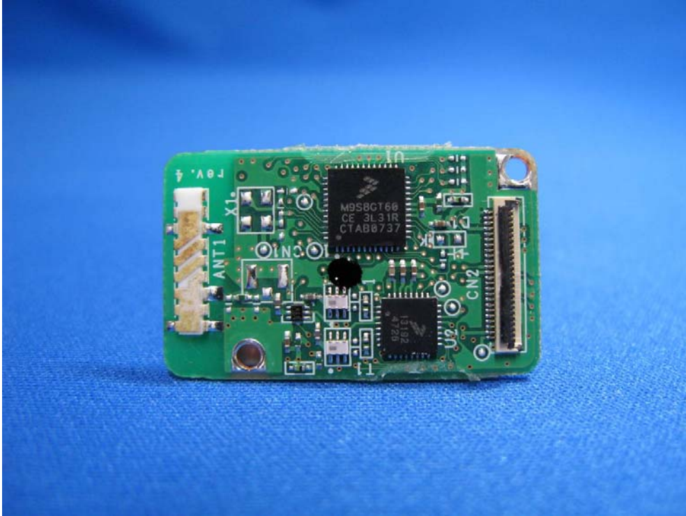
WDT-6M RF module component side (Same as WDT-5E)
