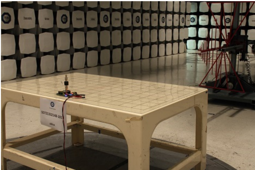
Radiated Emissions Below 1GHz Rear
