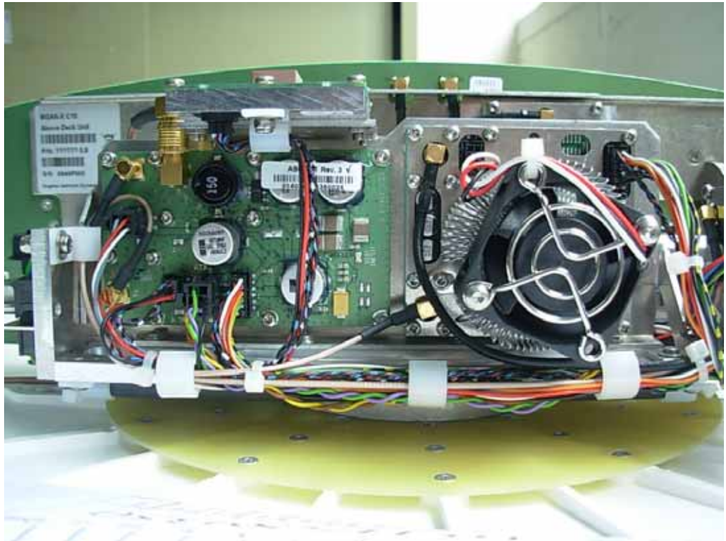
FIGURE 25 INMARSAT BGAN LVUT (M/N: GX-10) SATELLITE ANTENNA – INSIDE REAR VIEW
