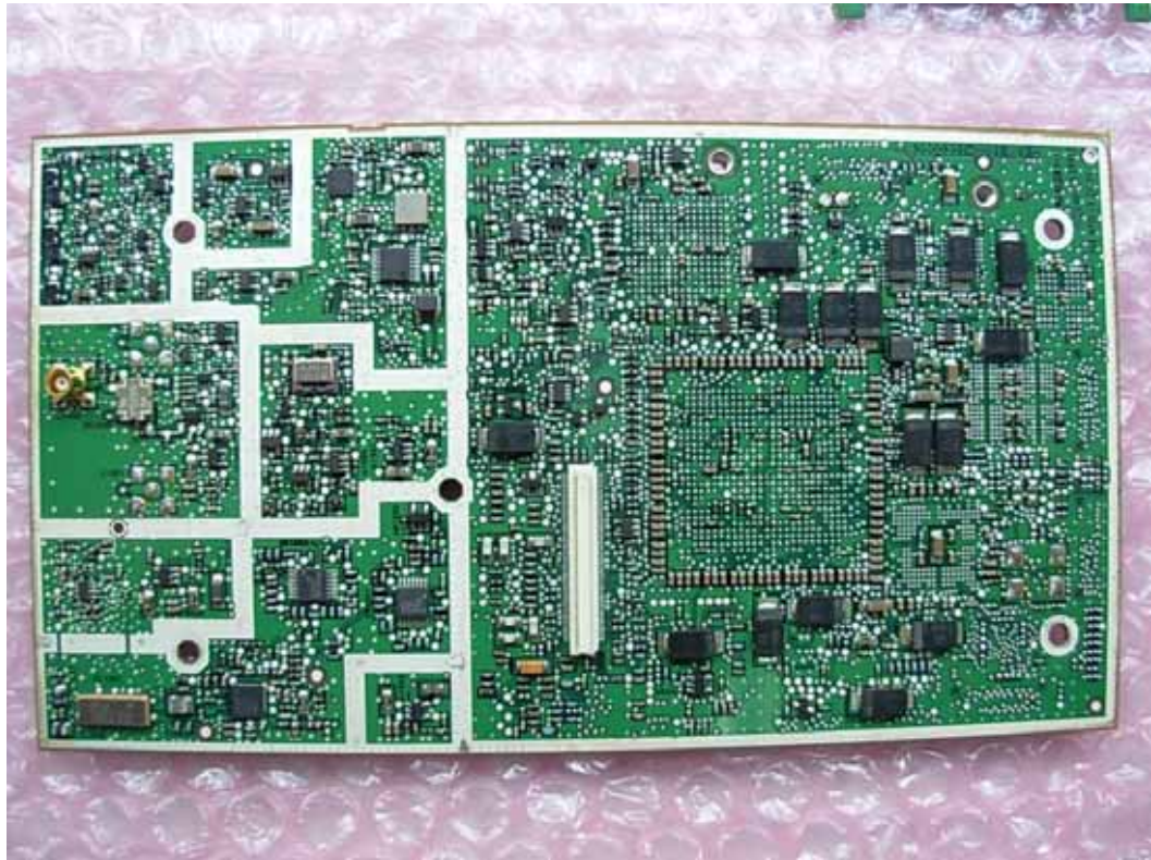
FIGURE 15 INMARSAT BGAN LVUT (M/N: GX-10) MAIN BOARD - MODULE – SIDE 2
