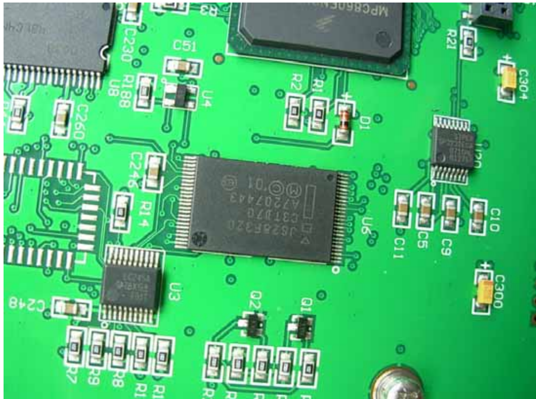
FIGURE 9 INMARSAT BGAN LVUT (M/N: GX-10) MAIN BOARD – IC 5
