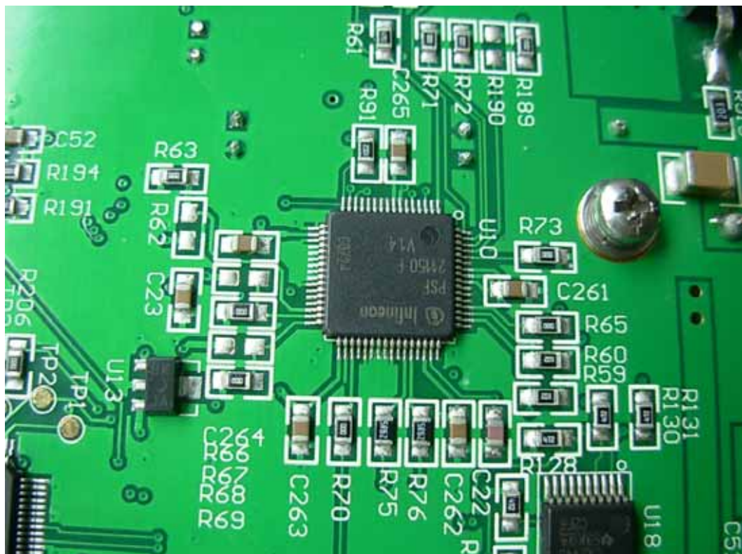
FIGURE 8 INMARSAT BGAN LVUT (M/N: GX-10) MAIN BOARD – IC 4
