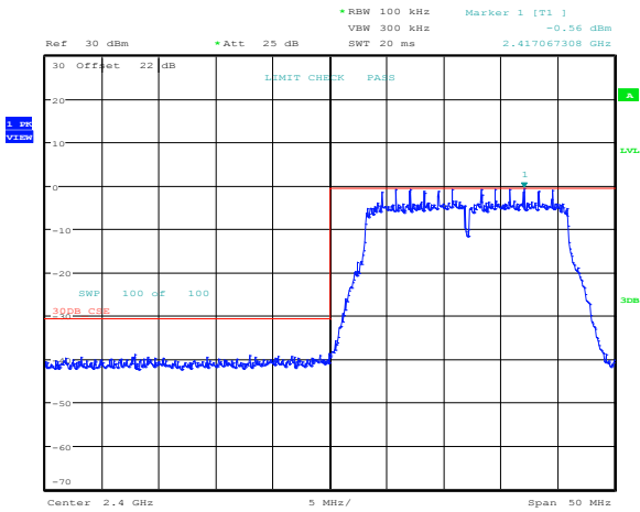
Figure 8.3-45: Band edge emission outside restricted bands at 2.4 GHz for 802.11b, 1 Mbps
