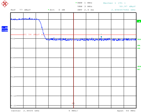
Figure 8.3-98: Cabinet radiation at the restricted band edge at 2.4835 GHz for 802.11n HT20
