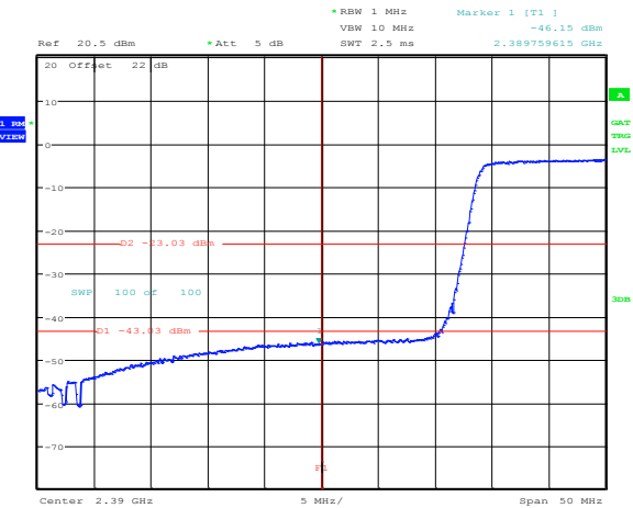
Figure 8.3-74: Band edge emission within restricted bands at 2.4 GHz for 802.11n HT20, MCS 7, average
