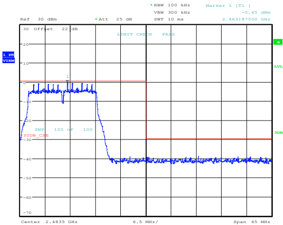
Figure 8.3-53: Band edge emission outside restricted bands at 2.4835 GHz for 802.11b, 1 Mbps
