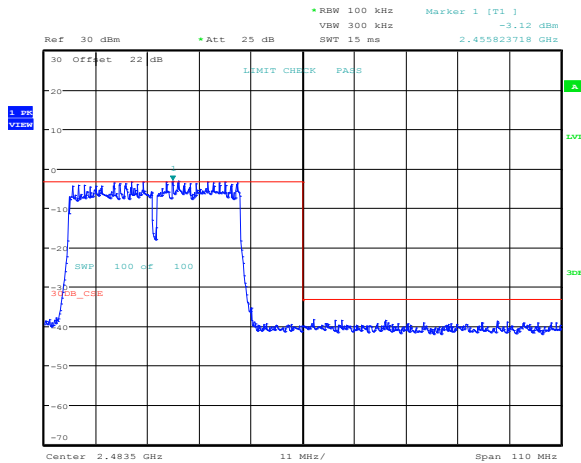
Figure 8.3-58: Band edge emission outside restricted bands at 2.4835 GHz for 802.11g, 54 Mbps
