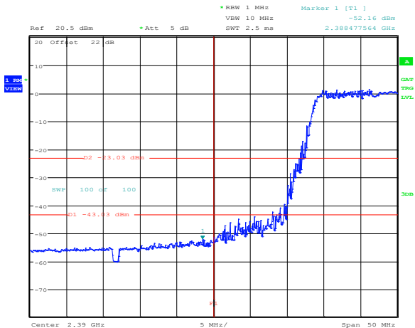
Figure 8.3-62: Band edge emission within restricted bands at 2.4 GHz for 802.11b, 1 Mbps, average
