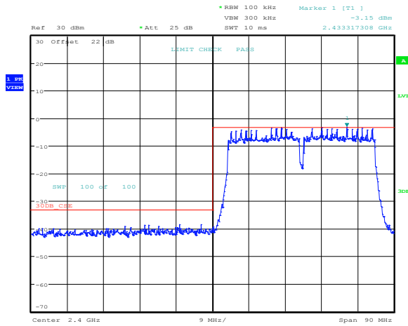
Figure 8.3-46: Band edge emission outside restricted bands at 2.4 GHz for 802.11g, 6 Mbps
