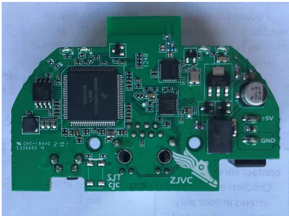
PCB front
