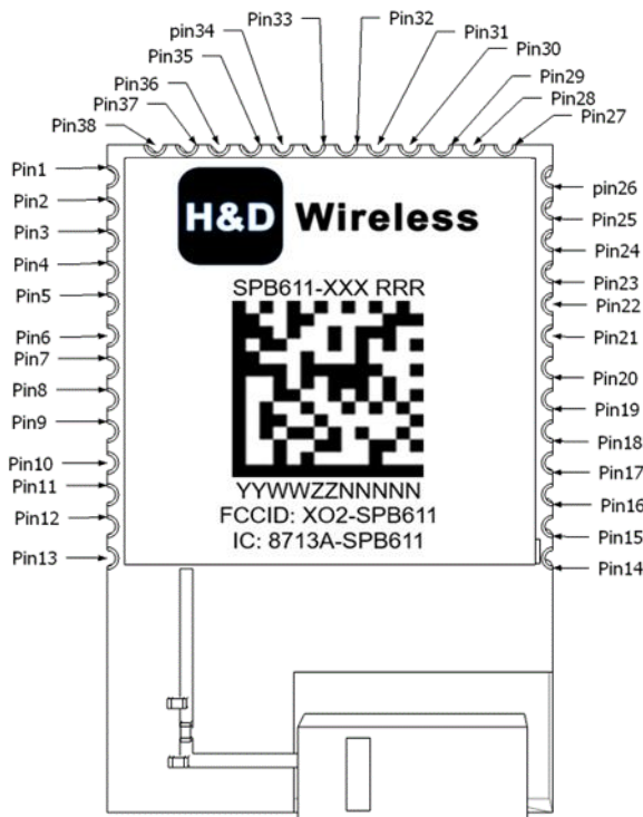
Figure 4-2: SPB611-Bxxx package pin out, top view.
