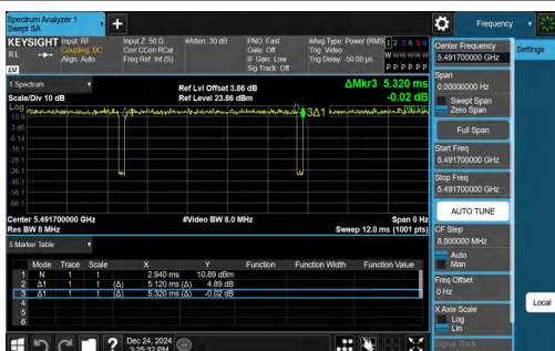
NTNV-11AX20SISO-Ant1-5500-106Tone-RU53
