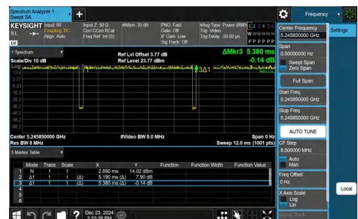
NTNV-11AX20SISO-Ant1-5260-26Tone-RU0
