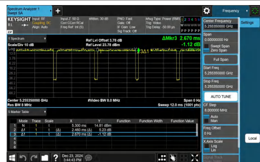
NTNV-11AX20SISO-Ant1-5300-52Tone-RU39
