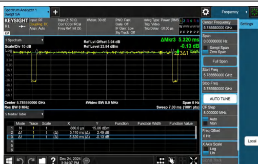
NTVN-11AX20SISO-Ant1-5785-106Tone-RU53
