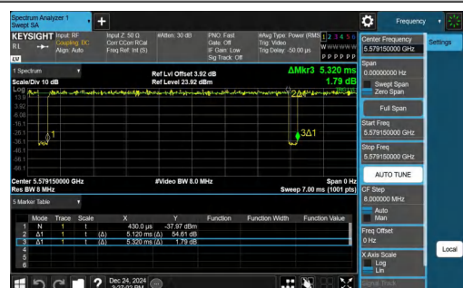
NTNV-11AX20SISO-Ant1-5580-106Tone-RU53
