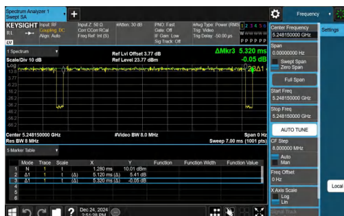
NTNV-11AX20SISO-Ant1-5240-106Tone-RU54
