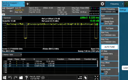
NTNV-11AX20SISO-Ant1-5180-106Tone-RU53
