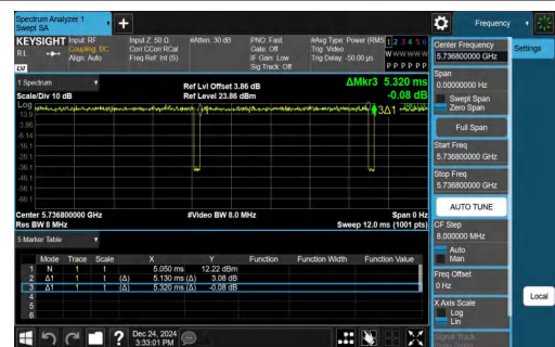
NTVN-11AX20SISO-Ant1-5745-106Tone-RU53
