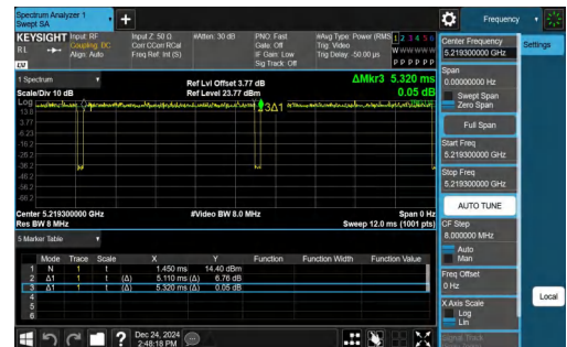
NTNV-11AX20SISO-Ant1-5220-106Tone-RU53
